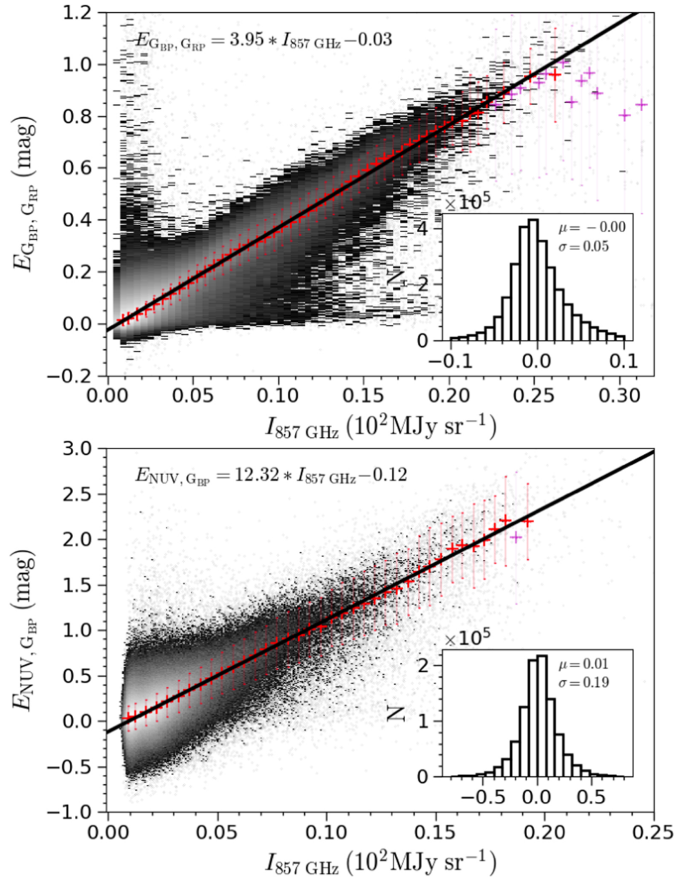
Figure 2. from The Extinction and Distance of the MBM Molecular Clouds at High Galactic Latitude null 2021 APJS 256 46 doi:10.3847/1538-4365/ac1601 http://dx.doi.org/10.3847/1538-4365/ac1601
