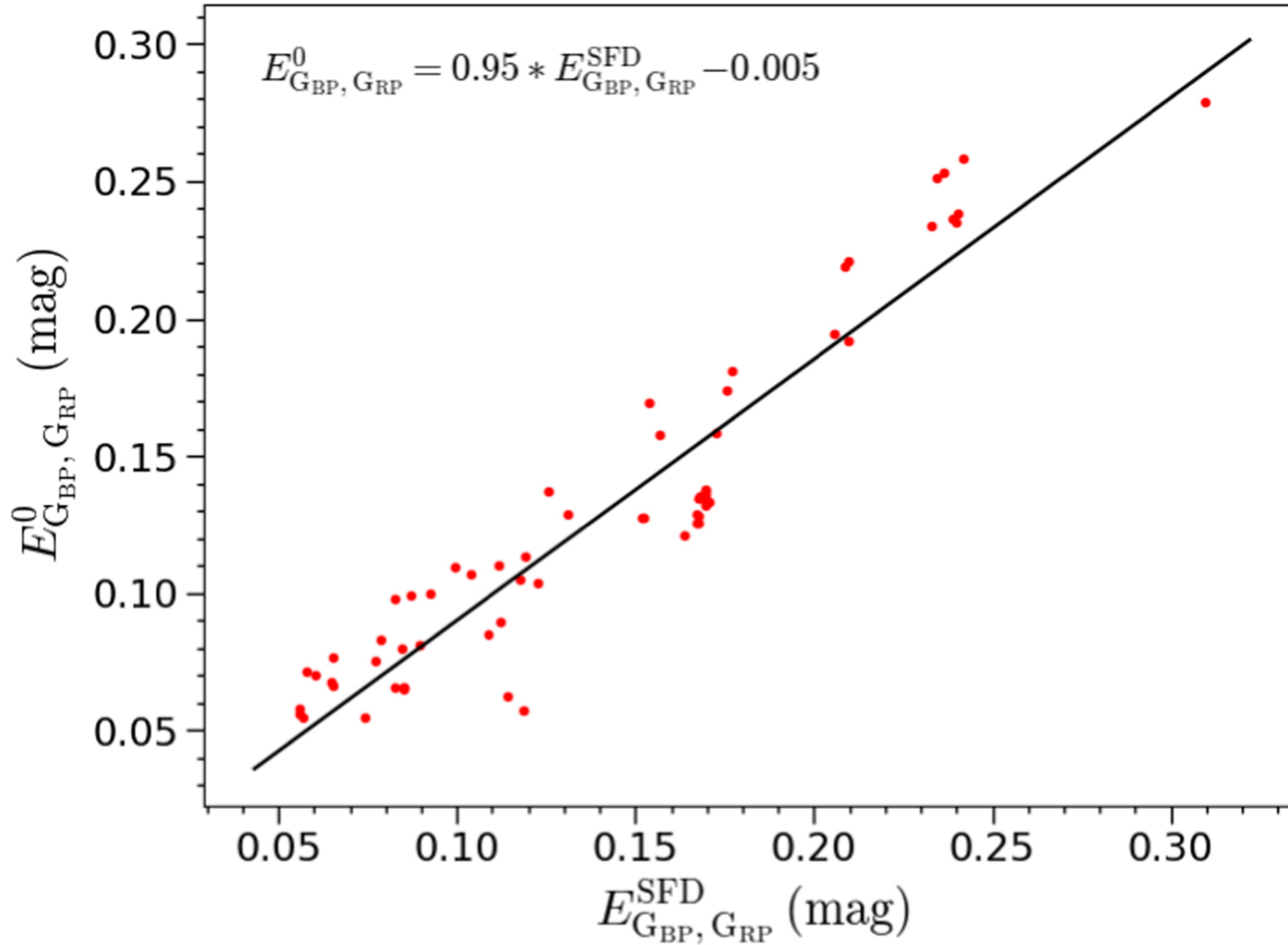
Figure 12. from The Extinction and Distance of the MBM Molecular Clouds at High Galactic Latitude null 2021 APJS 256 46 doi:10.3847/1538-4365/ac1601 http://dx.doi.org/10.3847/1538-4365/ac1601 © 2021. The Author(s). Published by the American Astronomical Society.
