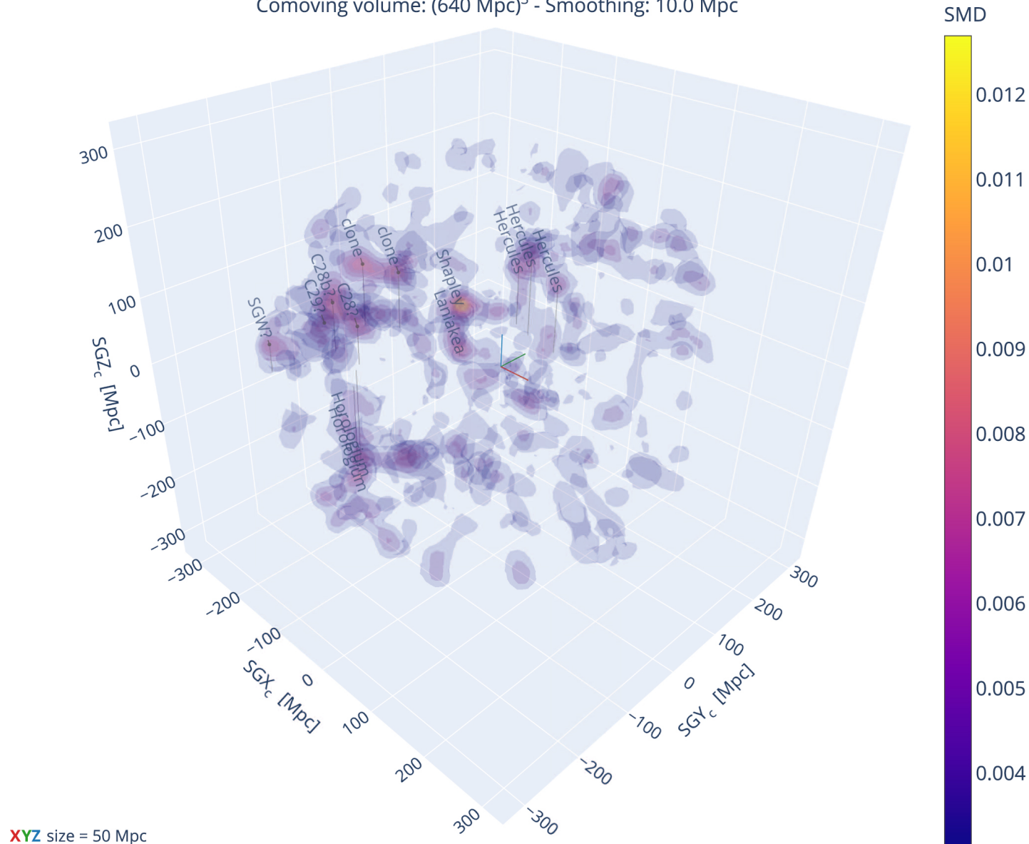
Figure 8. from Stellar Mass and Star Formation Rate within a Billion Light-years null 2021 APJS 256 15 doi:10.3847/1538-4365/ac09f5 https://dx.doi.org/10.3847/1538-4365/ac09f5 © 2021. The American Astronomical Society. All rights reserved.
