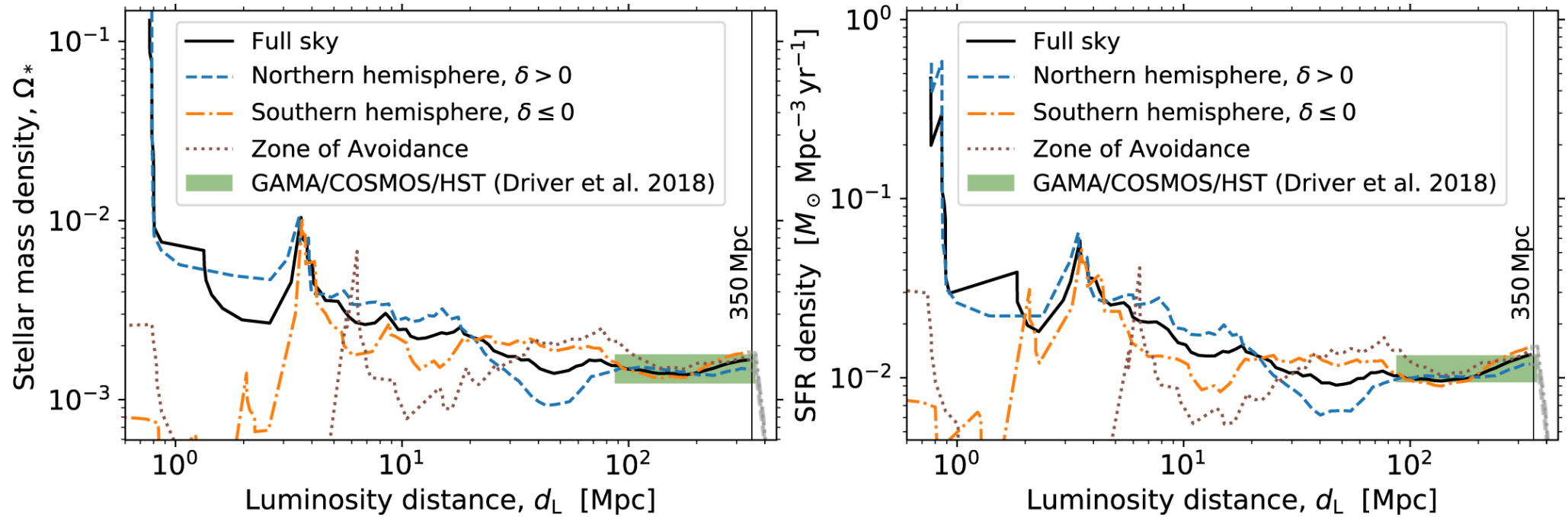
Figure 6. from Stellar Mass and Star Formation Rate within a Billion Light-years null 2021 APJS 256 15 doi:10.3847/1538-4365/ac09f5 https://dx.doi.org/10.3847/1538-4365/ac09f5 © 2021. The American Astronomical Society. All rights reserved.
