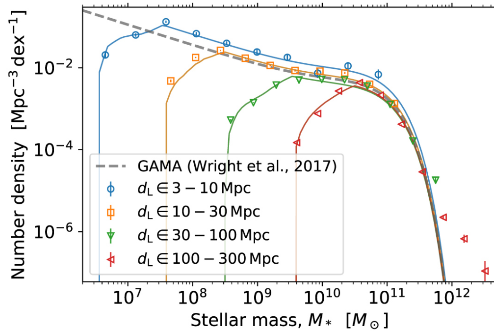
Figure 4. from Stellar Mass and Star Formation Rate within a Billion Light-years null 2021 APJS 256 15 doi:10.3847/1538-4365/ac09f5 https://dx.doi.org/10.3847/1538-4365/ac09f5 © 2021. The American Astronomical Society. All rights reserved.
