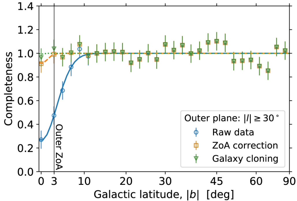
Figure 3. from Stellar Mass and Star Formation Rate within a Billion Light-years null 2021 APJS 256 15 doi:10.3847/1538-4365/ac09f5 https://dx.doi.org/10.3847/1538-4365/ac09f5 © 2021. The American Astronomical Society. All rights reserved.
