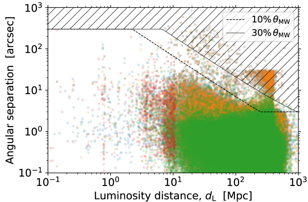
Figure 1. from Stellar Mass and Star Formation Rate within a Billion Light-years null 2021 APJS 256 15 doi:10.3847/1538-4365/ac09f5 https://dx.doi.org/10.3847/1538-4365/ac09f5 © 2021. The American Astronomical Society. All rights reserved.
