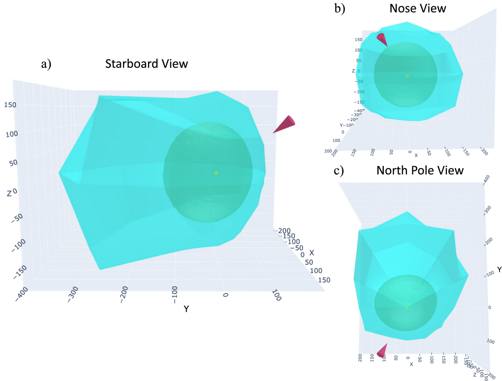
Figure 8. from A Three-dimensional Map of the Heliosphere from IBEX null 2021 APJS 254 40 doi:10.3847/1538-4365/abf658 https://dx.doi.org/10.3847/1538-4365/abf658 © 2021. The American Astronomical Society. All rights reserved.
