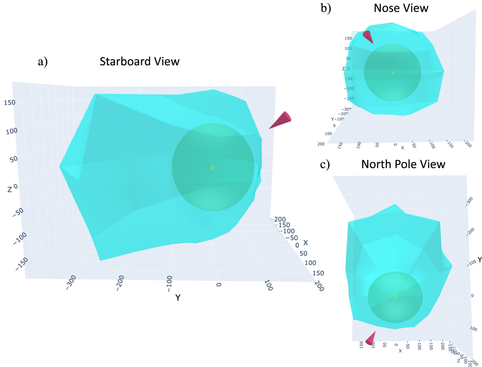
Figure 6. from A Three-dimensional Map of the Heliosphere from IBEX null 2021 APJS 254 40 doi:10.3847/1538-4365/abf658 https://dx.doi.org/10.3847/1538-4365/abf658 © 2021. The American Astronomical Society. All rights reserved.
