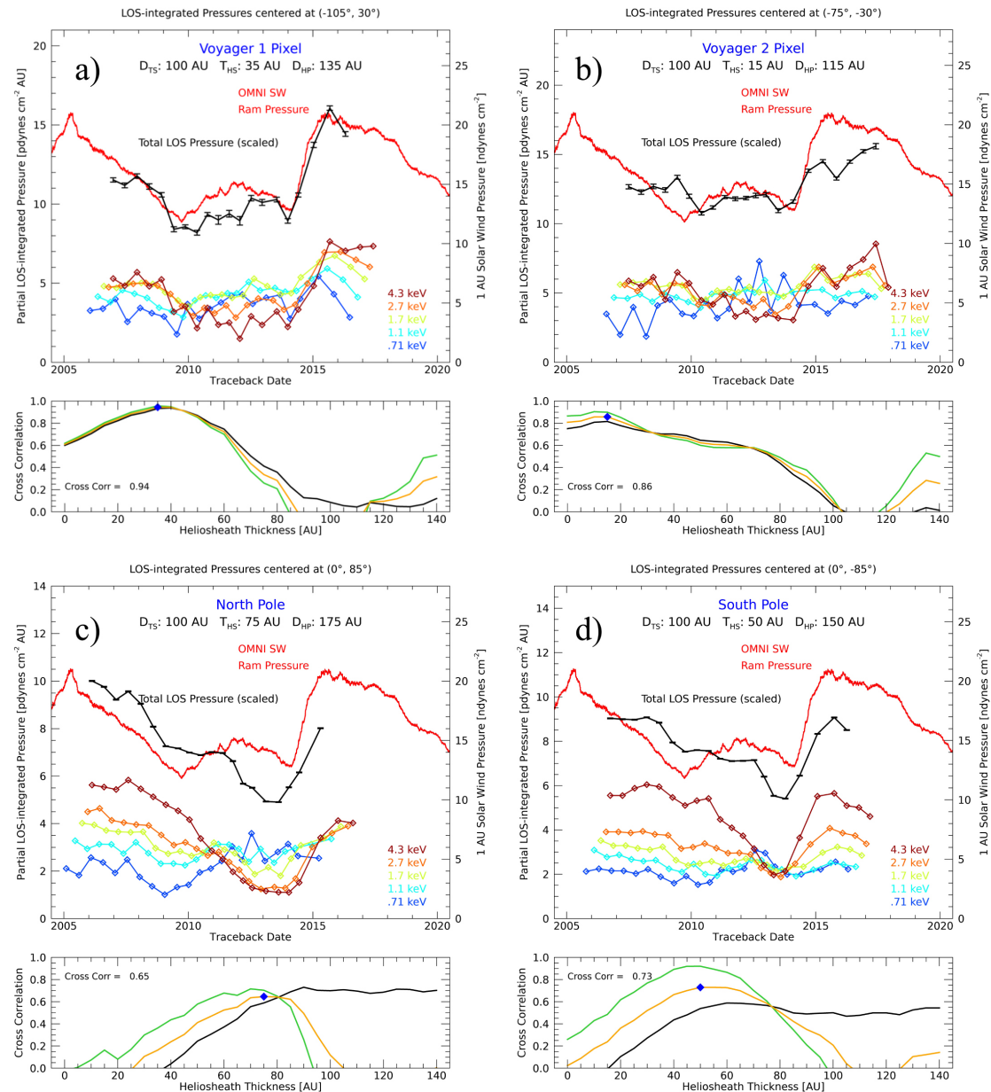
Figure 5. from A Three-dimensional Map of the Heliosphere from IBEX null 2021 APJS 254 40 doi:10.3847/1538-4365/abf658 https://dx.doi.org/10.3847/1538-4365/abf658 © 2021. The American Astronomical Society. All rights reserved.
