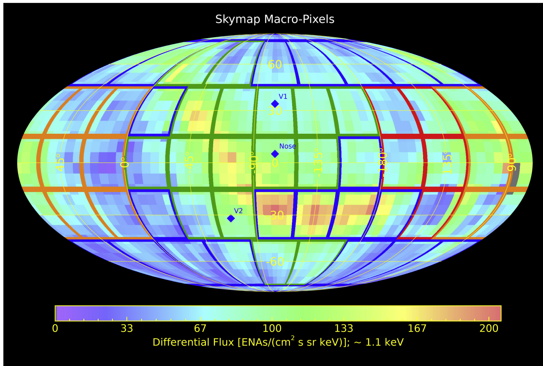
Figure 2. from A Three-dimensional Map of the Heliosphere from IBEX null 2021 APJS 254 40 doi:10.3847/1538-4365/abf658 https://dx.doi.org/10.3847/1538-4365/abf658 © 2021. The American Astronomical Society. All rights reserved.
