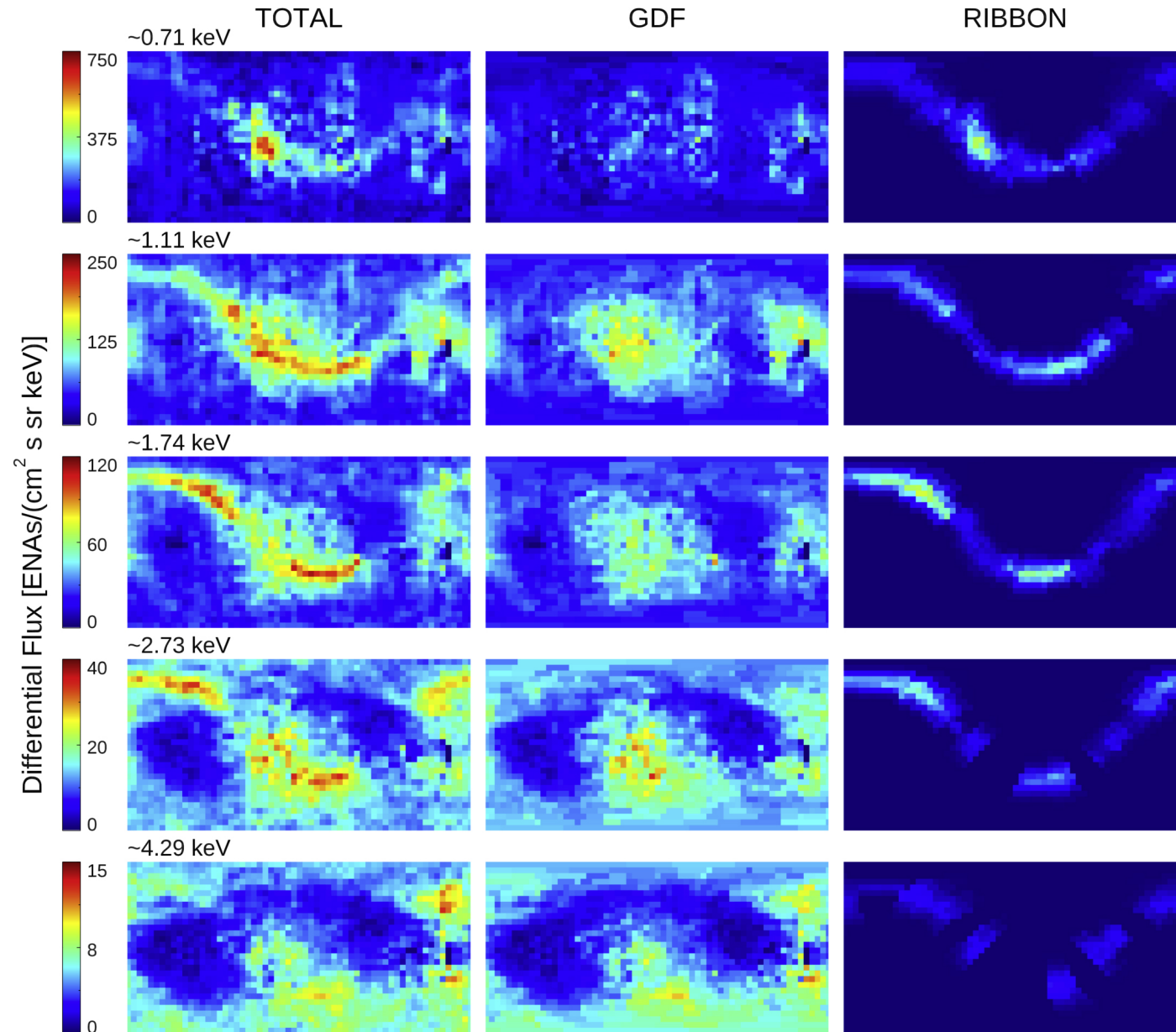
Figure 1. from A Three-dimensional Map of the Heliosphere from IBEX null 2021 APJS 254 40 doi:10.3847/1538-4365/abf658 https://dx.doi.org/10.3847/1538-4365/abf658 © 2021. The American Astronomical Society. All rights reserved.
