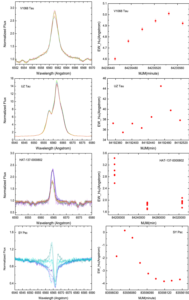
Figure 9. from Chromospheric Activity of Periodic Variable Stars Based on the LAMOST Low- and Medium-resolution Spectral Survey null 2021 APJS 253 51 doi:10.3847/1538-4365/abe30b https://dx.doi.org/10.3847/1538-4365/abe30b © 2021. The American Astronomical Society. All rights reserved.
