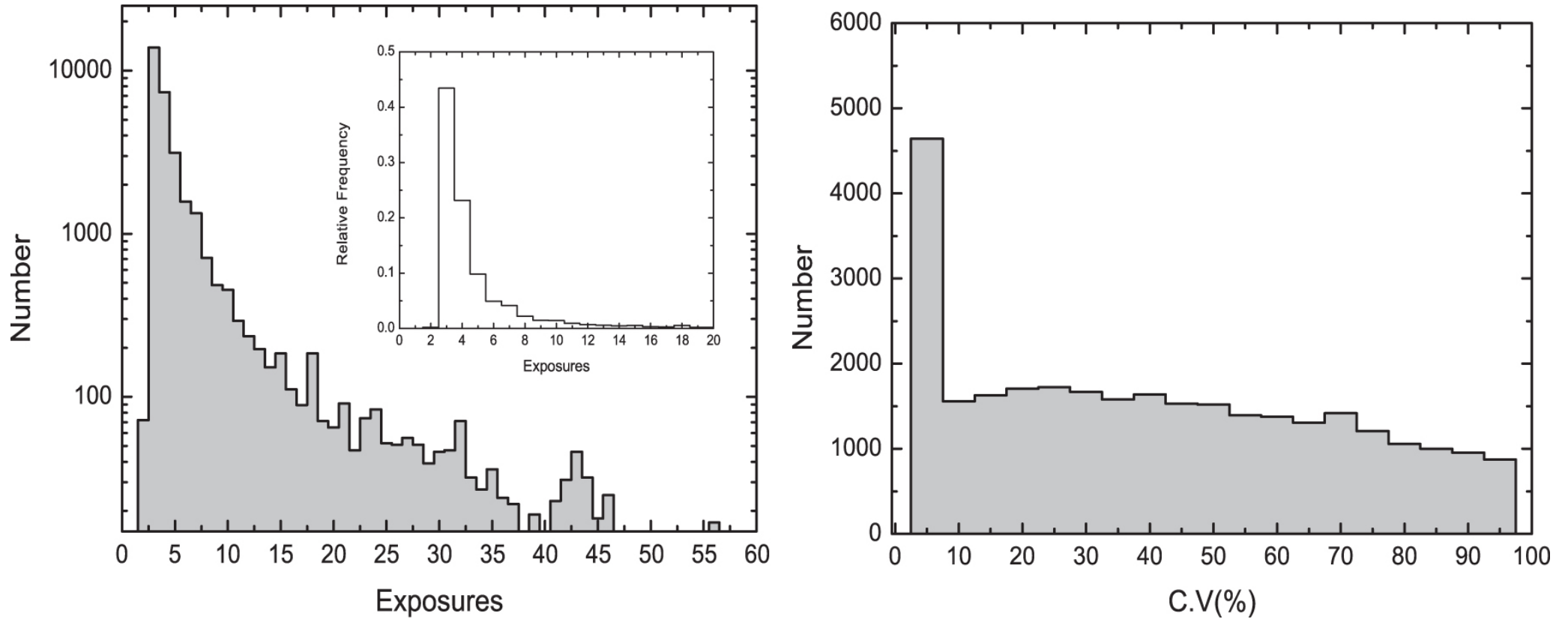
Figure 8. from Chromospheric Activity of Periodic Variable Stars Based on the LAMOST Low- and Medium-resolution Spectral Survey null 2021 APJS 253 51 doi:10.3847/1538-4365/abe30b https://dx.doi.org/10.3847/1538-4365/abe30b © 2021. The American Astronomical Society. All rights reserved.
