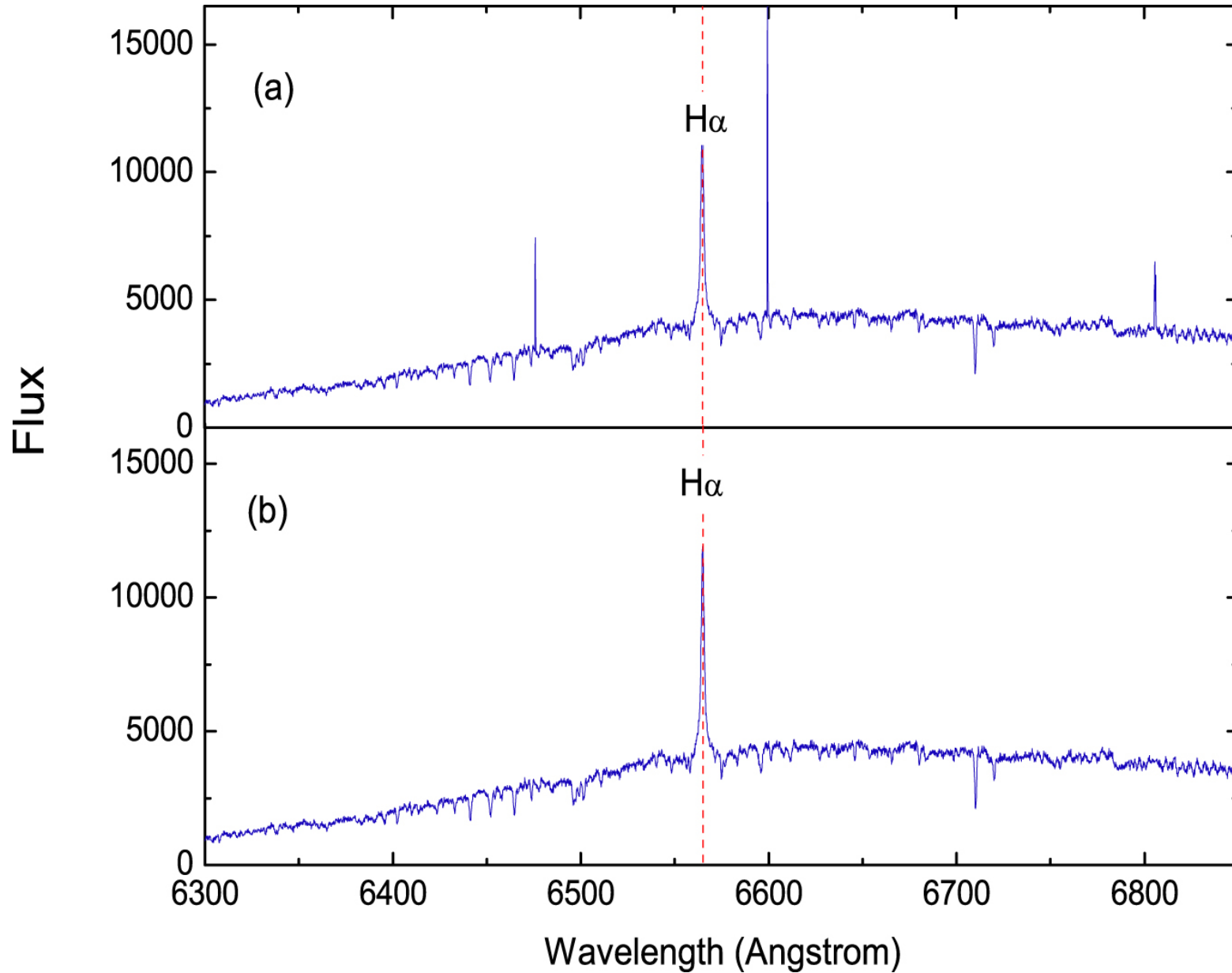
Figure 5. from Chromospheric Activity of Periodic Variable Stars Based on the LAMOST Low- and Medium-resolution Spectral Survey null 2021 APJS 253 51 doi:10.3847/1538-4365/abe30b http://dx.doi.org/10.3847/1538-4365/abe30b © 2021. The American Astronomical Society. All rights reserved.
