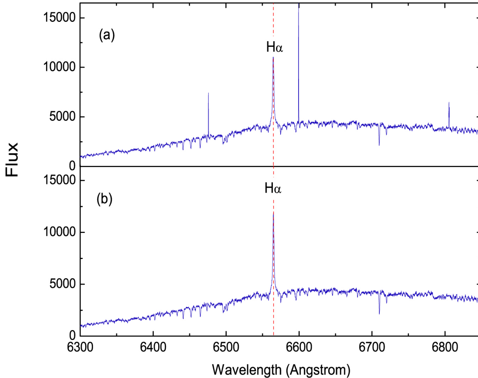
Figure 5. from Chromospheric Activity of Periodic Variable Stars Based on the LAMOST Low- and Medium-resolution Spectral Survey null 2021 APJS 253 51 doi:10.3847/1538-4365/abe30b https://dx.doi.org/10.3847/1538-4365/abe30b © 2021. The American Astronomical Society. All rights reserved.
