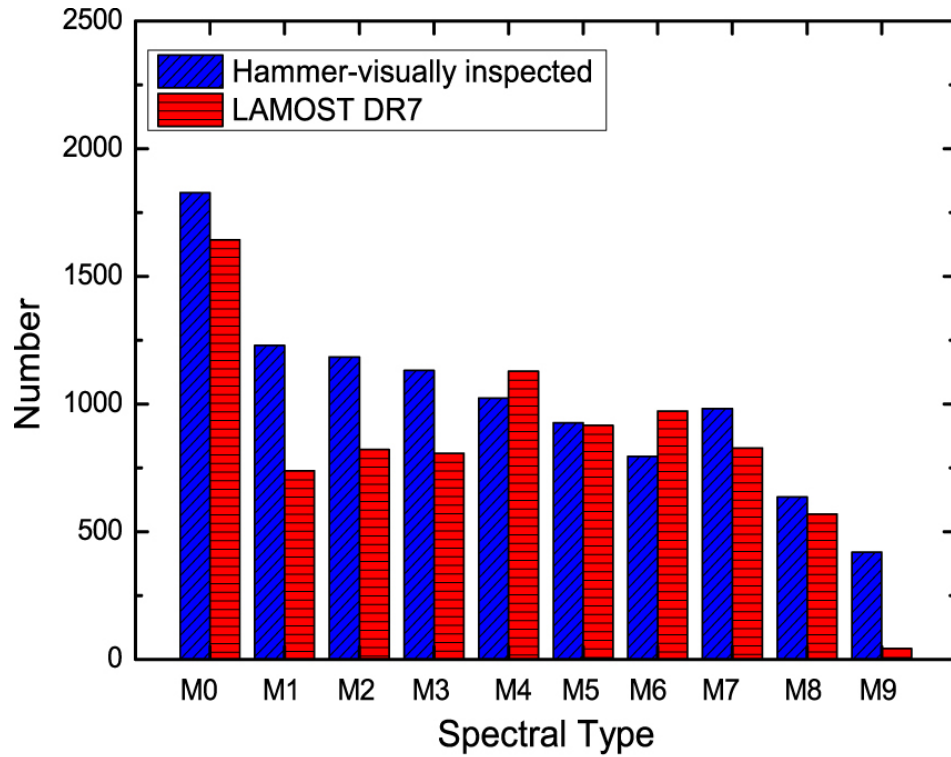
Figure 4. from Chromospheric Activity of Periodic Variable Stars Based on the LAMOST Low- and Medium-resolution Spectral Survey null 2021 APJS 253 51 doi:10.3847/1538-4365/abe30b https://dx.doi.org/10.3847/1538-4365/abe30b
