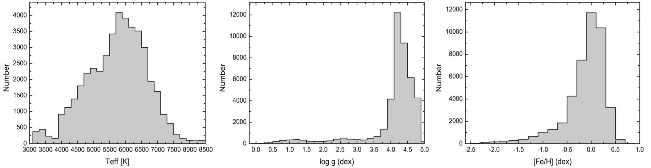
Figure 3. from Chromospheric Activity of Periodic Variable Stars Based on the LAMOST Low- and Medium-resolution Spectral Survey null 2021 APJS 253 51 doi:10.3847/1538-4365/abe30b http://dx.doi.org/10.3847/1538-4365/abe30b © 2021. The American Astronomical Society. All rights reserved.
