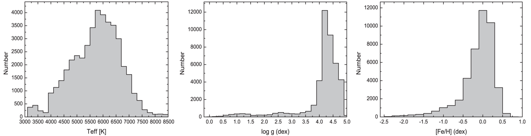
Figure 3. from Chromospheric Activity of Periodic Variable Stars Based on the LAMOST Low- and Medium-resolution Spectral Survey null 2021 APJS 253 51 doi:10.3847/1538-4365/abe30b https://dx.doi.org/10.3847/1538-4365/abe30b © 2021. The American Astronomical Society. All rights reserved.
