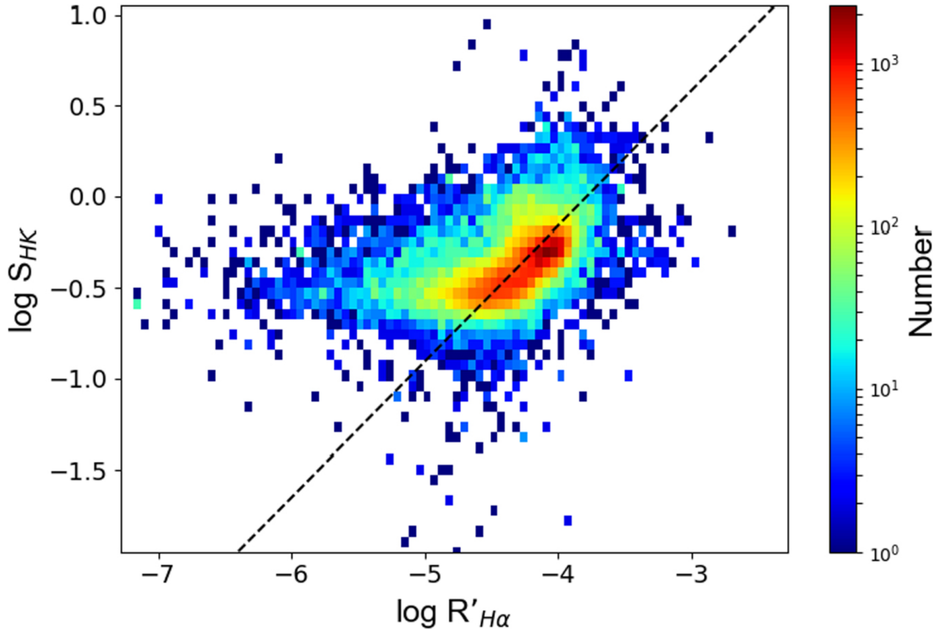
Figure 20. from Chromospheric Activity of Periodic Variable Stars Based on the LAMOST Low- and Medium-resolution Spectral Survey null 2021 APJS 253 51 doi:10.3847/1538-4365/abe30b http://dx.doi.org/10.3847/1538-4365/abe30b © 2021. The American Astronomical Society. All rights reserved.
