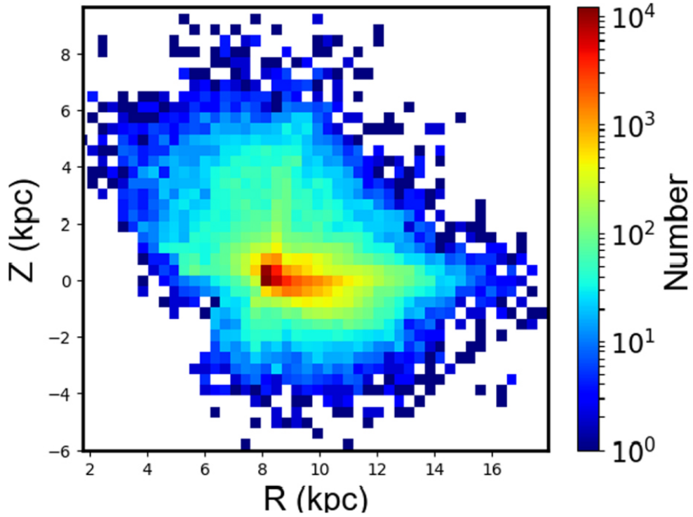
Figure 2. from Chromospheric Activity of Periodic Variable Stars Based on the LAMOST Low- and Medium-resolution Spectral Survey null 2021 APJS 253 51 doi:10.3847/1538-4365/abe30b http://dx.doi.org/10.3847/1538-4365/abe30b © 2021. The American Astronomical Society. All rights reserved.
