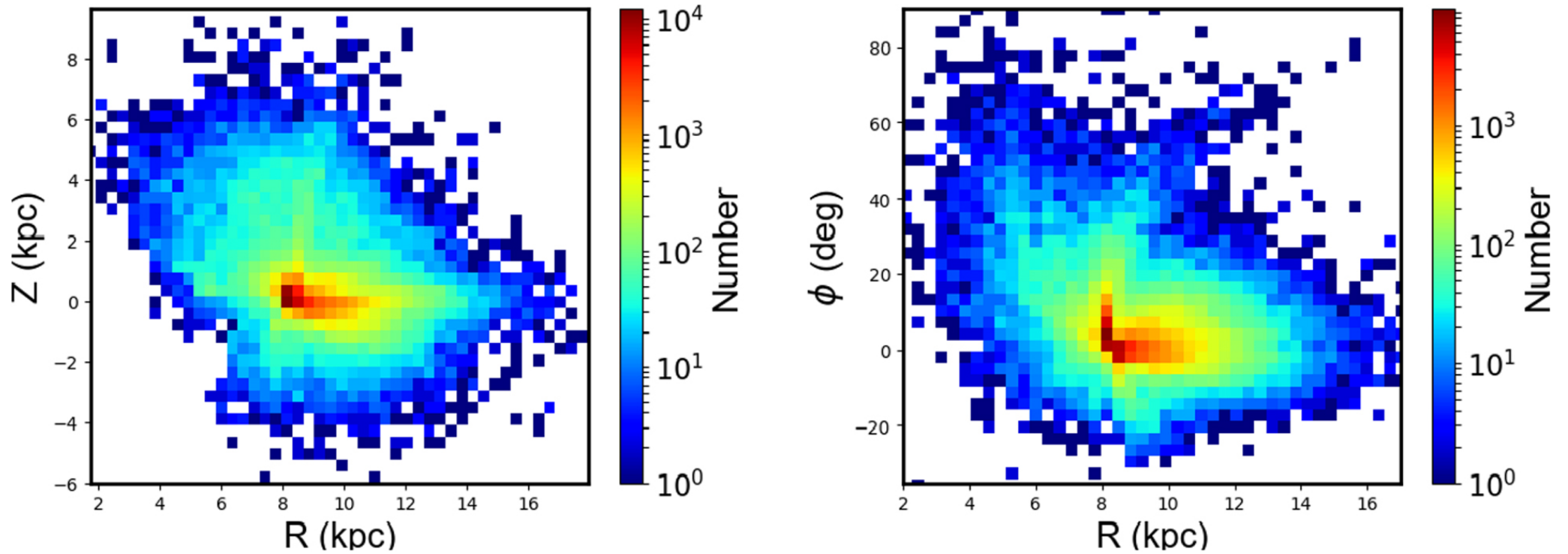
Figure 2. from Chromospheric Activity of Periodic Variable Stars Based on the LAMOST Low- and Medium-resolution Spectral Survey null 2021 APJS 253 51 doi:10.3847/1538-4365/abe30b https://dx.doi.org/10.3847/1538-4365/abe30b © 2021. The American Astronomical Society. All rights reserved.
