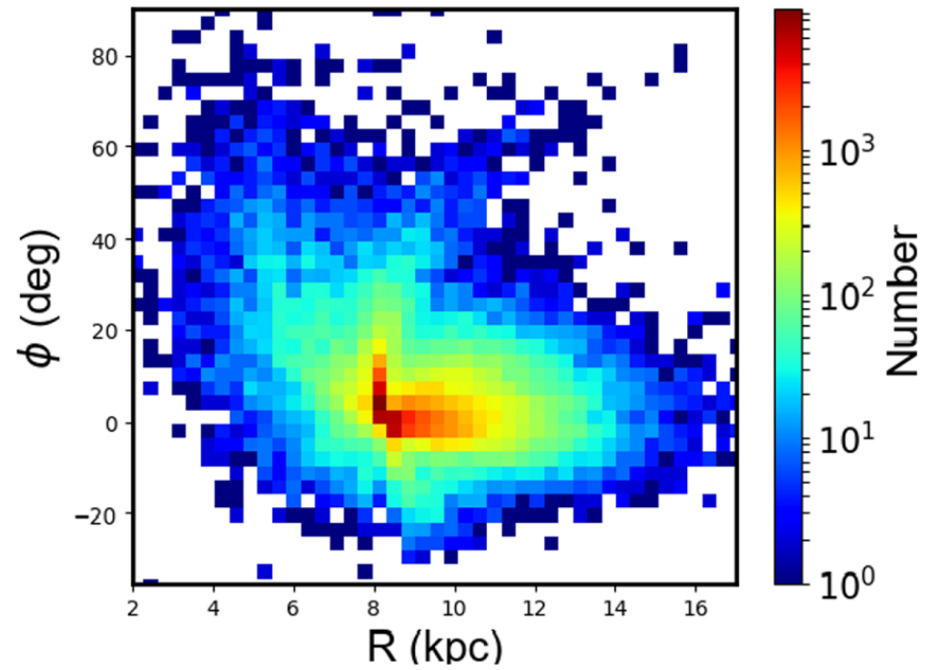
Figure 2. from Chromospheric Activity of Periodic Variable Stars Based on the LAMOST Low- and Medium-resolution Spectral Survey null 2021 APJS 253 51 doi:10.3847/1538-4365/abe30b http://dx.doi.org/10.3847/1538-4365/abe30b © 2021. The American Astronomical Society. All rights reserved.
