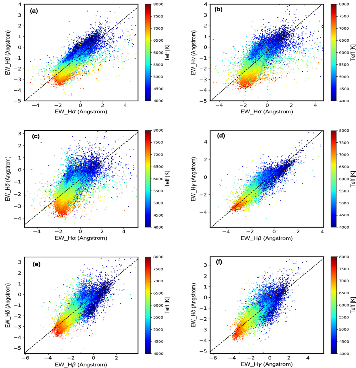
Figure 18. from Chromospheric Activity of Periodic Variable Stars Based on the LAMOST Low- and Medium-resolution Spectral Survey null 2021 APJS 253 51 doi:10.3847/1538-4365/abe30b https://dx.doi.org/10.3847/1538-4365/abe30b © 2021. The American Astronomical Society. All rights reserved.
