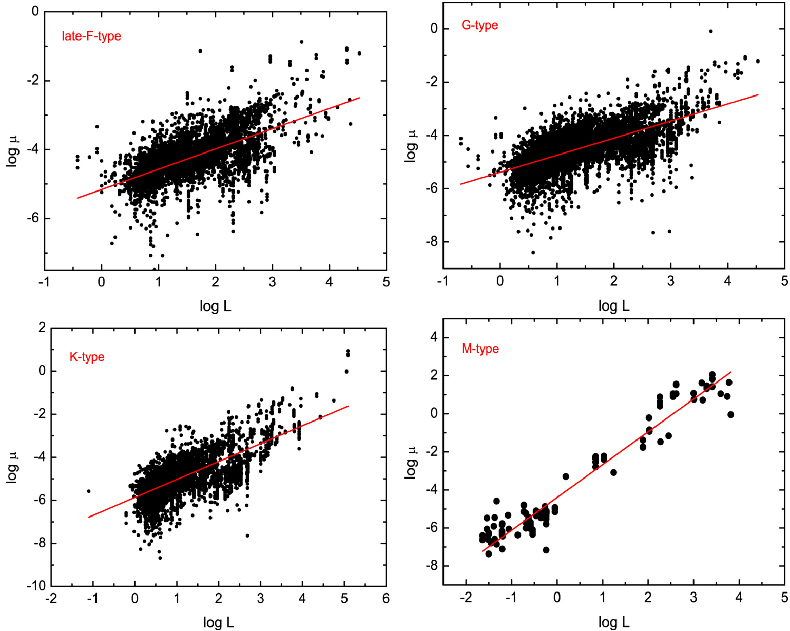
Figure 17. from Chromospheric Activity of Periodic Variable Stars Based on the LAMOST Low- and Medium-resolution Spectral Survey null 2021 APJS 253 51 doi:10.3847/1538-4365/abe30b http://dx.doi.org/10.3847/1538-4365/abe30b © 2021. The American Astronomical Society. All rights reserved.
