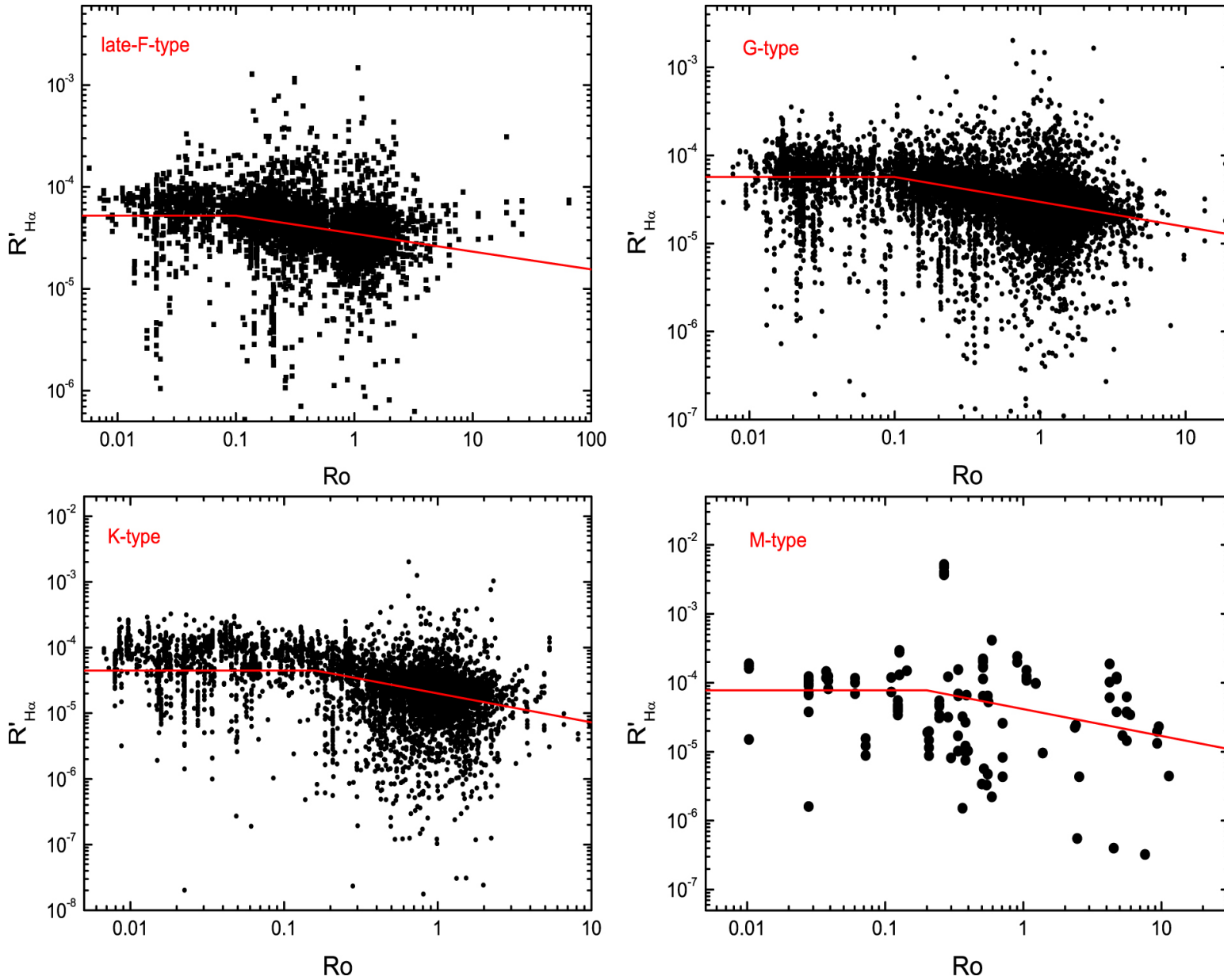
Figure 16. from Chromospheric Activity of Periodic Variable Stars Based on the LAMOST Low- and Medium-resolution Spectral Survey null 2021 APJS 253 51 doi:10.3847/1538-4365/abe30b http://dx.doi.org/10.3847/1538-4365/abe30b © 2021. The American Astronomical Society. All rights reserved.
