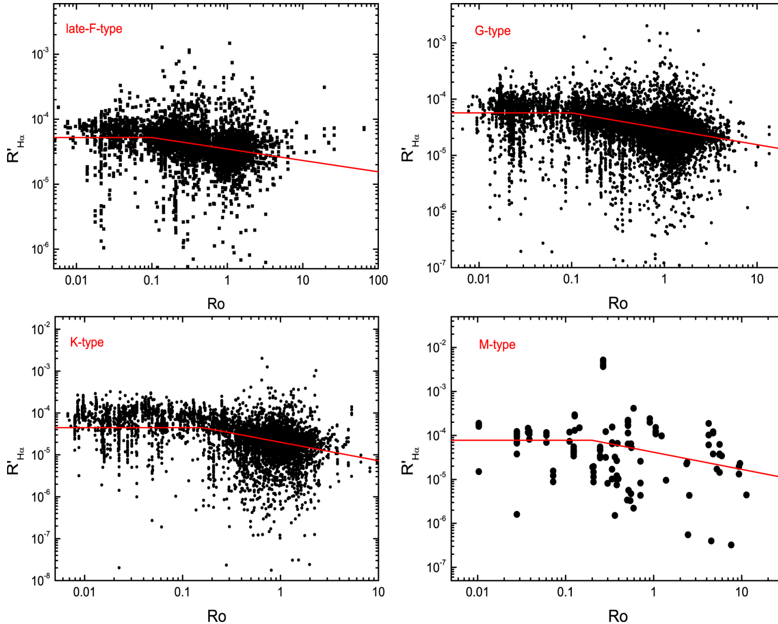
Figure 16. from Chromospheric Activity of Periodic Variable Stars Based on the LAMOST Low- and Medium-resolution Spectral Survey null 2021 APJS 253 51 doi:10.3847/1538-4365/abe30b https://dx.doi.org/10.3847/1538-4365/abe30b © 2021. The American Astronomical Society. All rights reserved.
