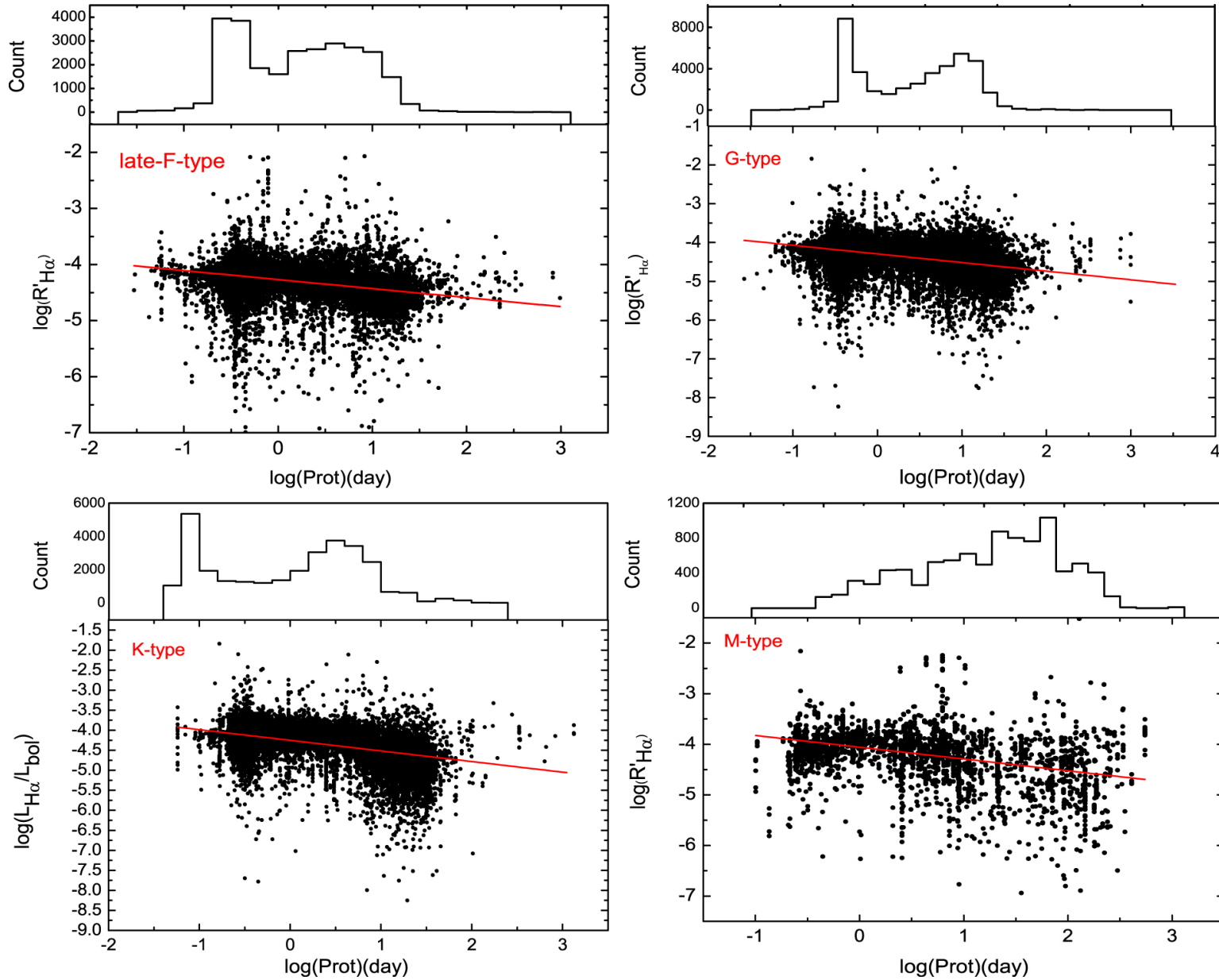
Figure 15. from Chromospheric Activity of Periodic Variable Stars Based on the LAMOST Low- and Medium-resolution Spectral Survey null 2021 APJS 253 51 doi:10.3847/1538-4365/abe30b http://dx.doi.org/10.3847/1538-4365/abe30b
