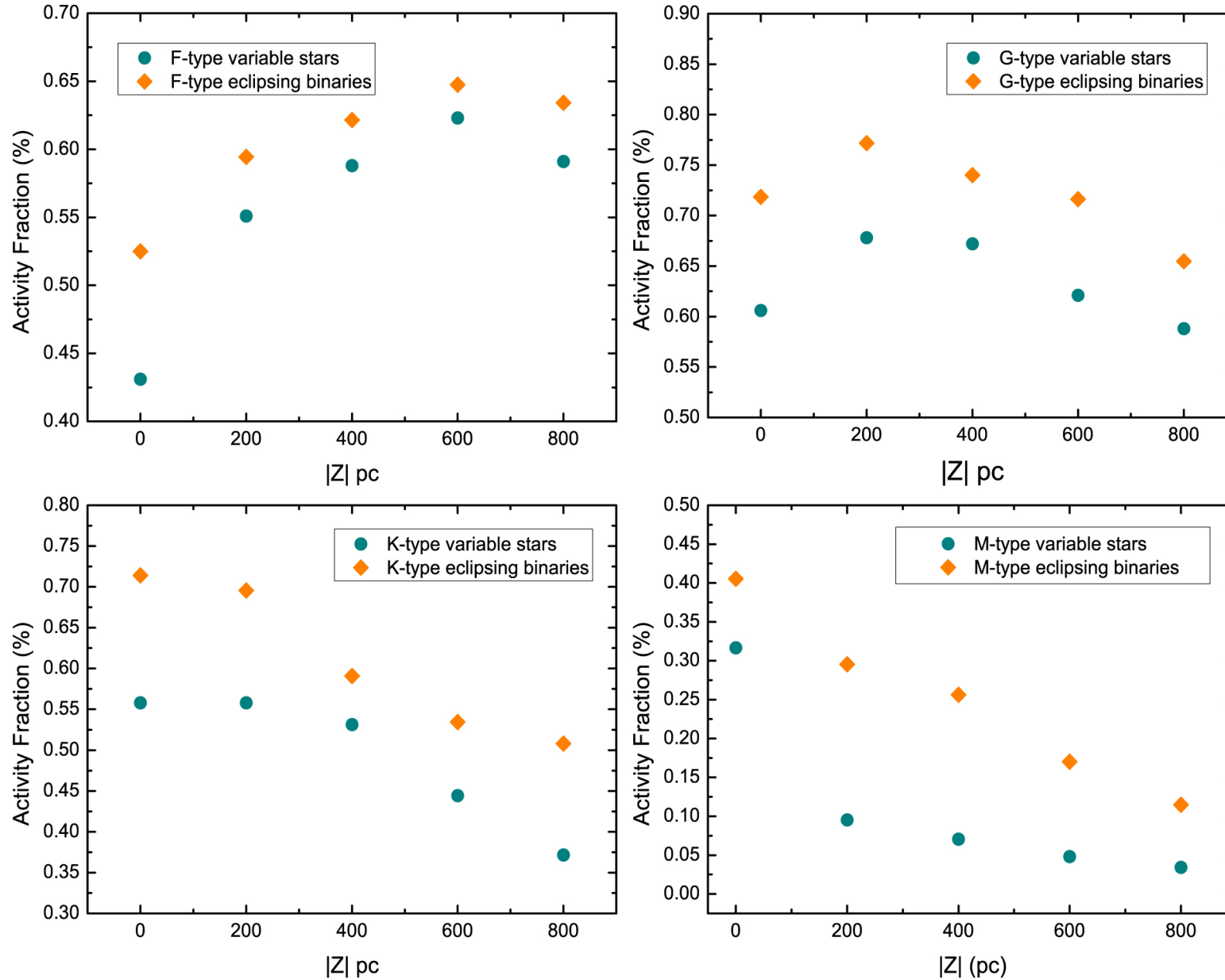
Figure 14. from Chromospheric Activity of Periodic Variable Stars Based on the LAMOST Low- and Medium-resolution Spectral Survey null 2021 APJS 253 51 doi:10.3847/1538-4365/abe30b http://dx.doi.org/10.3847/1538-4365/abe30b
