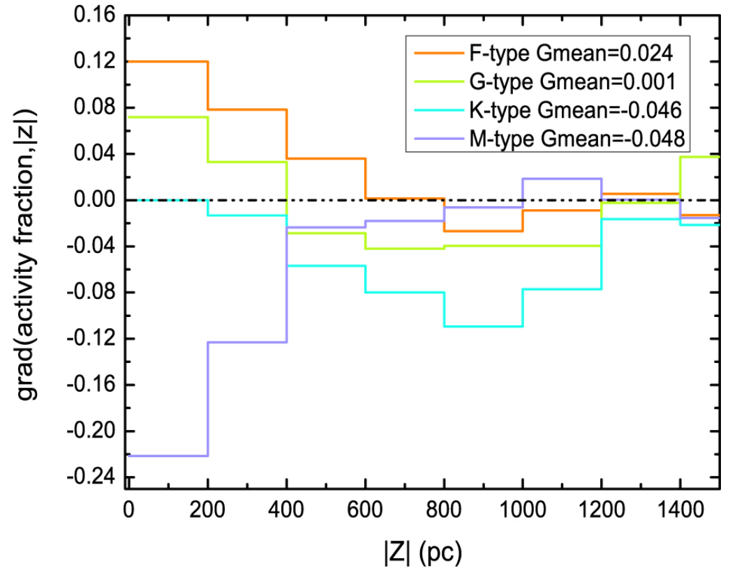
Figure 13. from Chromospheric Activity of Periodic Variable Stars Based on the LAMOST Low- and Medium-resolution Spectral Survey null 2021 APJS 253 51 doi:10.3847/1538-4365/abe30b http://dx.doi.org/10.3847/1538-4365/abe30b
