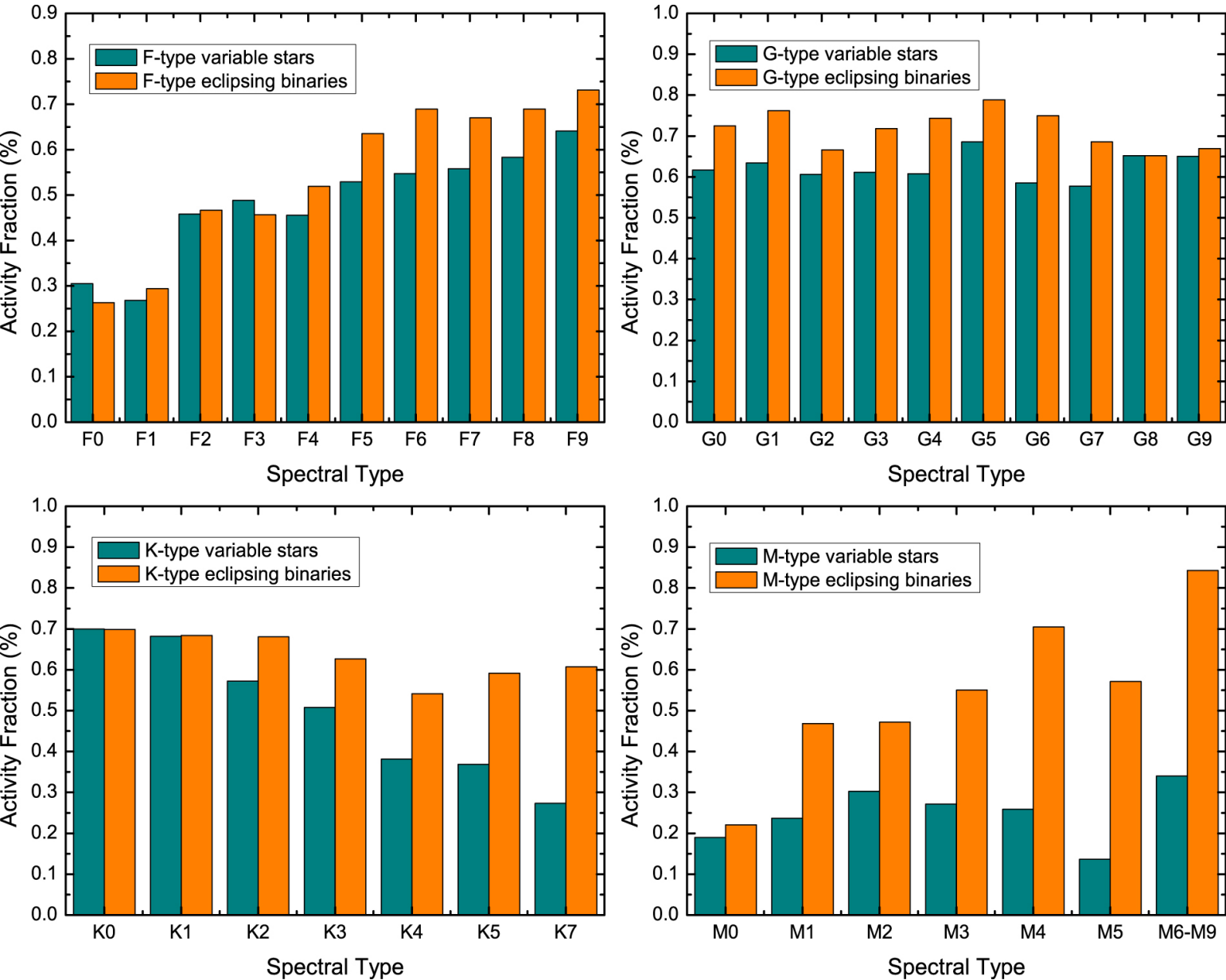
Figure 12. from Chromospheric Activity of Periodic Variable Stars Based on the LAMOST Low- and Medium-resolution Spectral Survey null 2021 APJS 253 51 doi:10.3847/1538-4365/abe30b https://dx.doi.org/10.3847/1538-4365/abe30b © 2021. The American Astronomical Society. All rights reserved.
