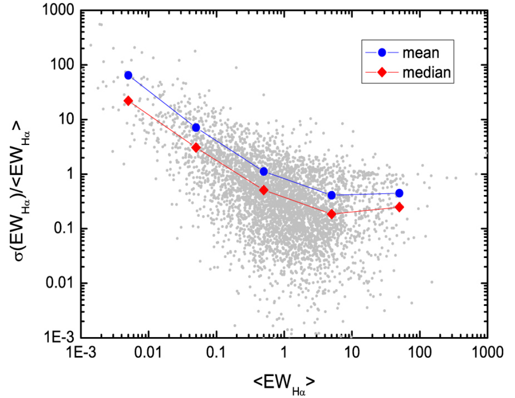
Figure 11. from Chromospheric Activity of Periodic Variable Stars Based on the LAMOST Low- and Medium-resolution Spectral Survey null 2021 APJS 253 51 doi:10.3847/1538-4365/abe30b http://dx.doi.org/10.3847/1538-4365/abe30b © 2021. The American Astronomical Society. All rights reserved.
