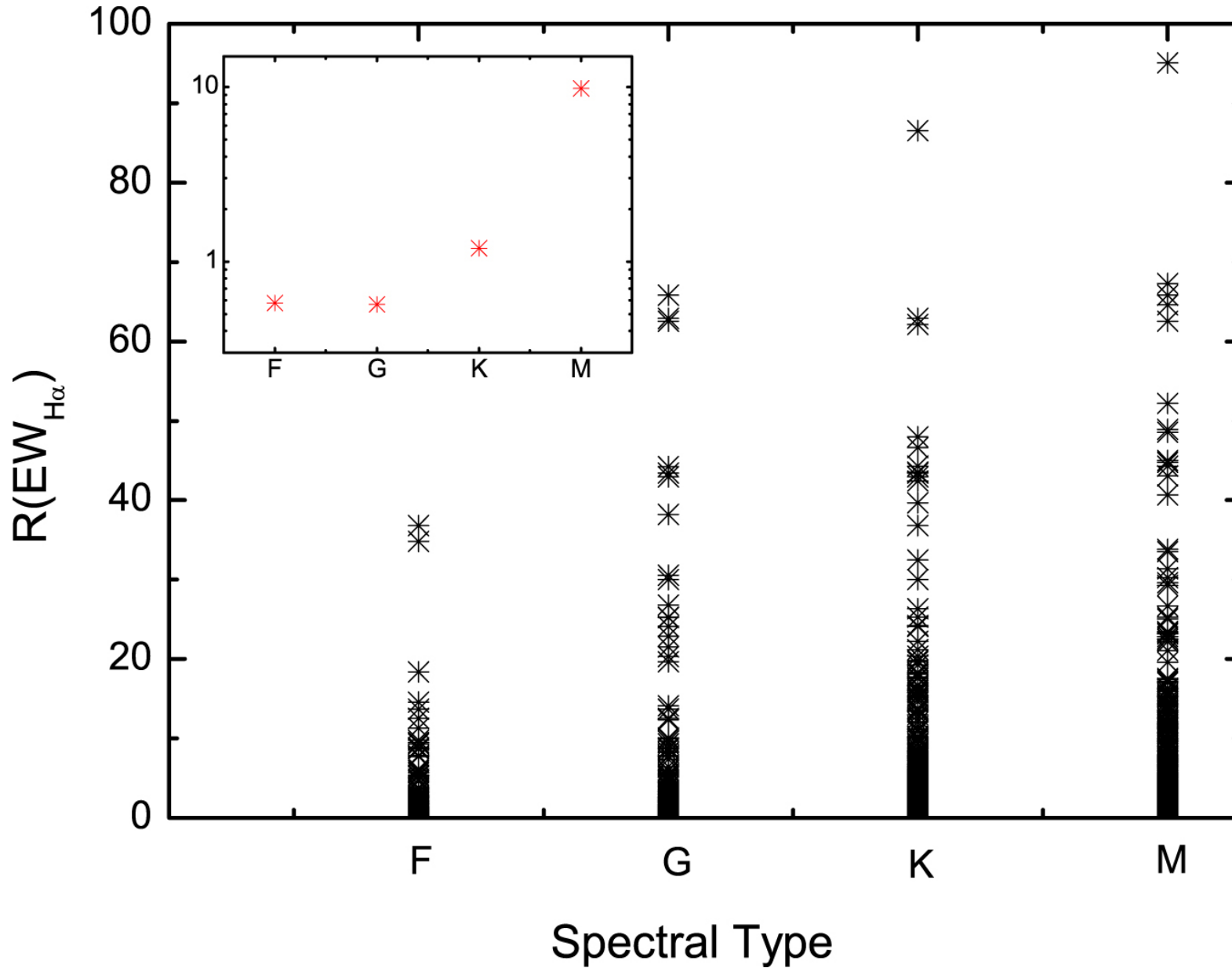
Figure 10. from Chromospheric Activity of Periodic Variable Stars Based on the LAMOST Low- and Medium-resolution Spectral Survey null 2021 APJS 253 51 doi:10.3847/1538-4365/abe30b http://dx.doi.org/10.3847/1538-4365/abe30b © 2021. The American Astronomical Society. All rights reserved.
