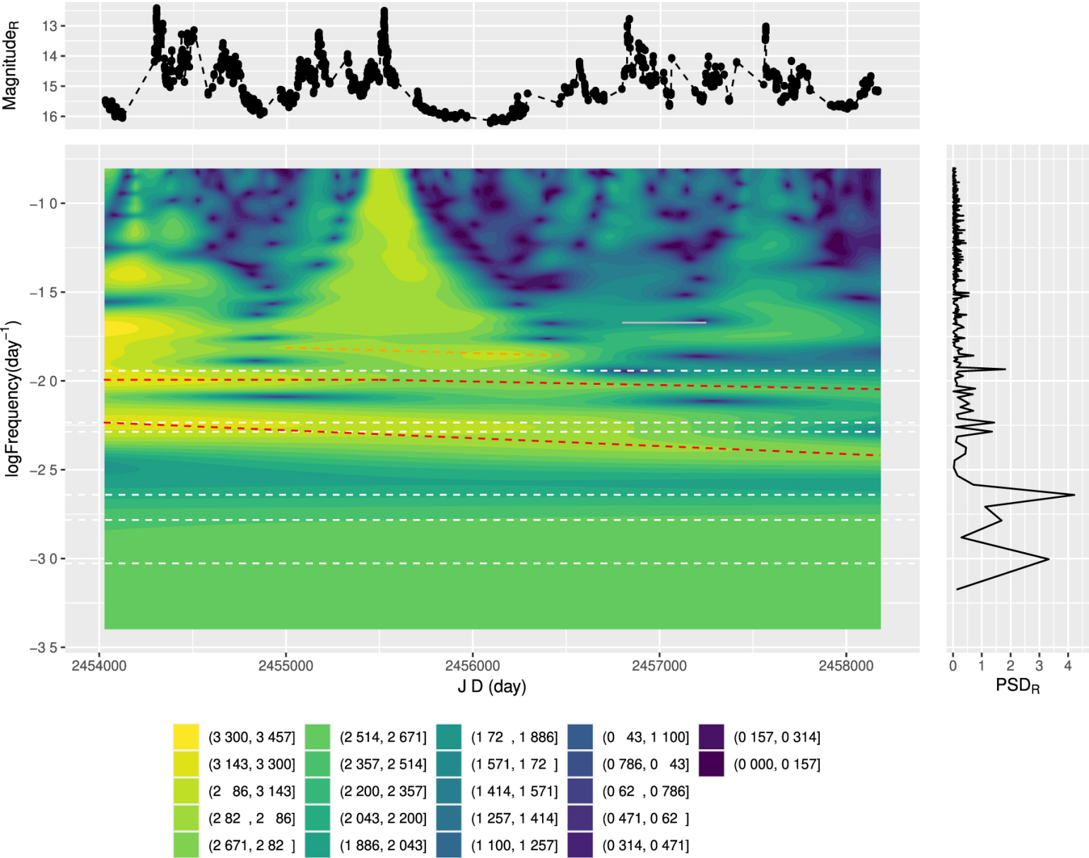
Figure 7. from Optical Photometry of the Quasar 3C 454.3 during the Period 2006–2018 and the Long-term Periodicity Analysis null 2021 APJS 253 10 doi:10.3847/1538-4365/abd32d https://dx.doi.org/10.3847/1538-4365/abd32d © 2021. The American Astronomical Society. All rights reserved.
