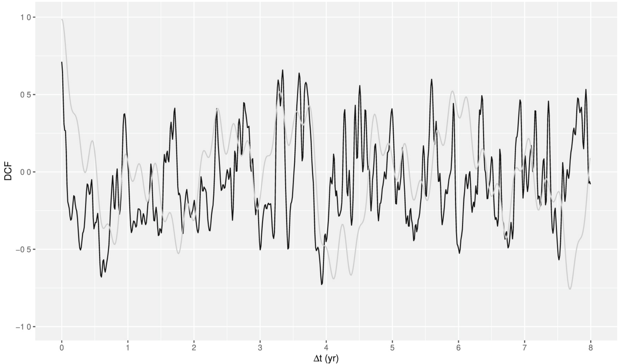
Figure 6. from Optical Photometry of the Quasar 3C 454.3 during the Period 2006–2018 and the Long-term Periodicity Analysis null 2021 APJS 253 10 doi:10.3847/1538-4365/abd32d https://dx.doi.org/10.3847/1538-4365/abd32d © 2021. The American Astronomical Society. All rights reserved.
