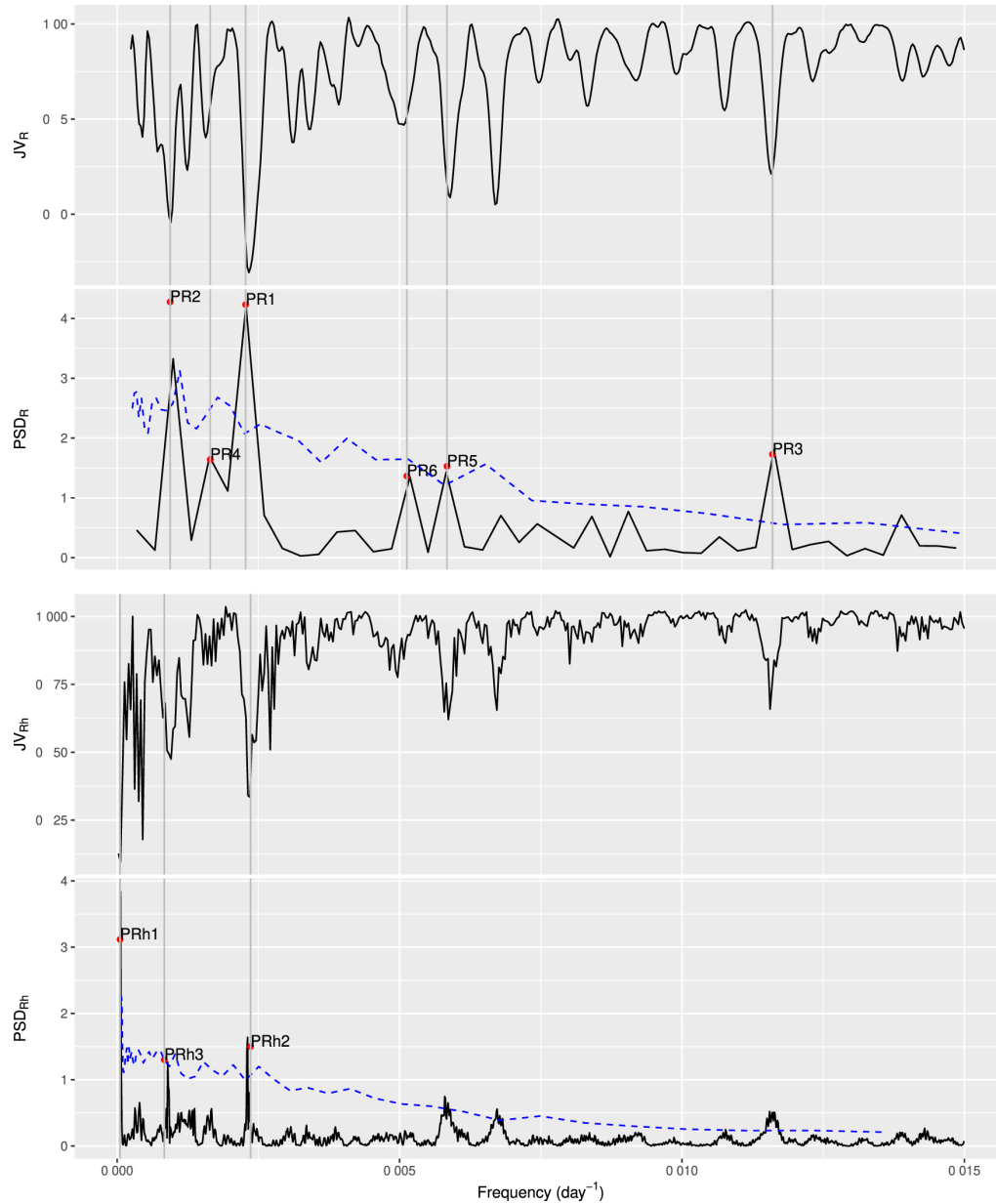
Figure 5. from Optical Photometry of the Quasar 3C 454.3 during the Period 2006–2018 and the Long-term Periodicity Analysis null 2021 APJS 253 10 doi:10.3847/1538-4365/abd32d https://dx.doi.org/10.3847/1538-4365/abd32d © 2021. The American Astronomical Society. All rights reserved.
