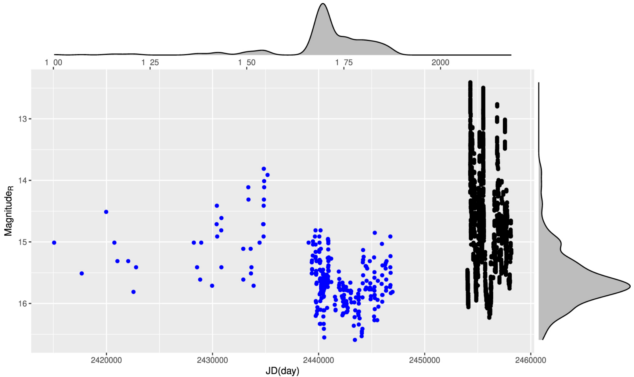
Figure 4. from Optical Photometry of the Quasar 3C 454.3 during the Period 2006–2018 and the Long-term Periodicity Analysis null 2021 APJS 253 10 doi:10.3847/1538-4365/abd32d https://dx.doi.org/10.3847/1538-4365/abd32d © 2021. The American Astronomical Society. All rights reserved.
