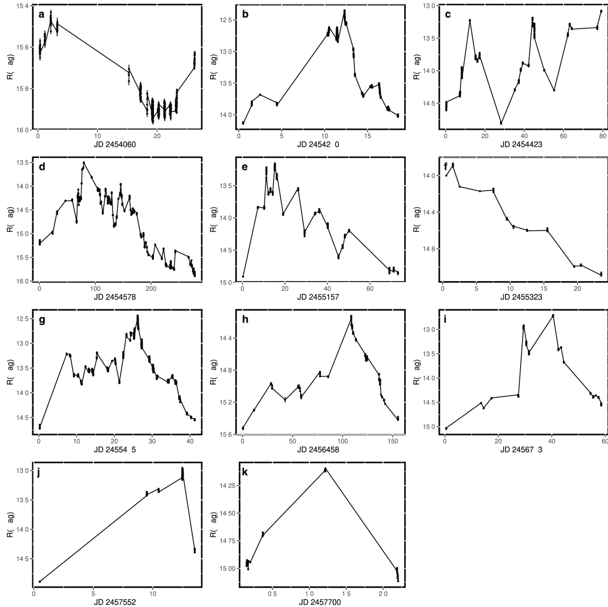
Figure 3. from Optical Photometry of the Quasar 3C 454.3 during the Period 2006–2018 and the Long-term Periodicity Analysis null 2021 APJS 253 10 doi:10.3847/1538-4365/abd32d https://dx.doi.org/10.3847/1538-4365/abd32d © 2021. The American Astronomical Society. All rights reserved.
