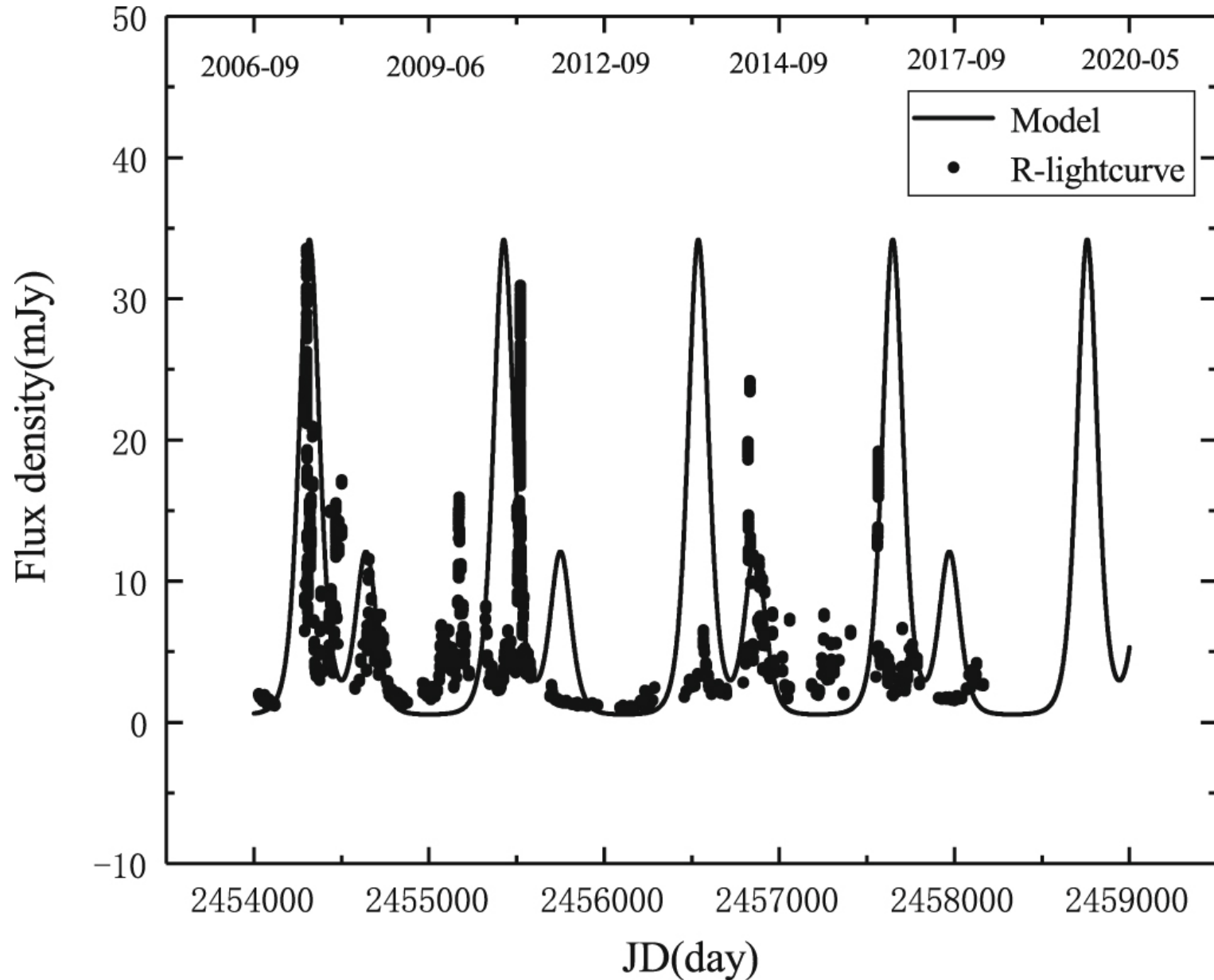
Figure 10. from Optical Photometry of the Quasar 3C 454.3 during the Period 2006–2018 and the Long-term Periodicity Analysis null 2021 APJS 253 10 doi:10.3847/1538-4365/abd32d https://dx.doi.org/10.3847/1538-4365/abd32d © 2021. The American Astronomical Society. All rights reserved.
