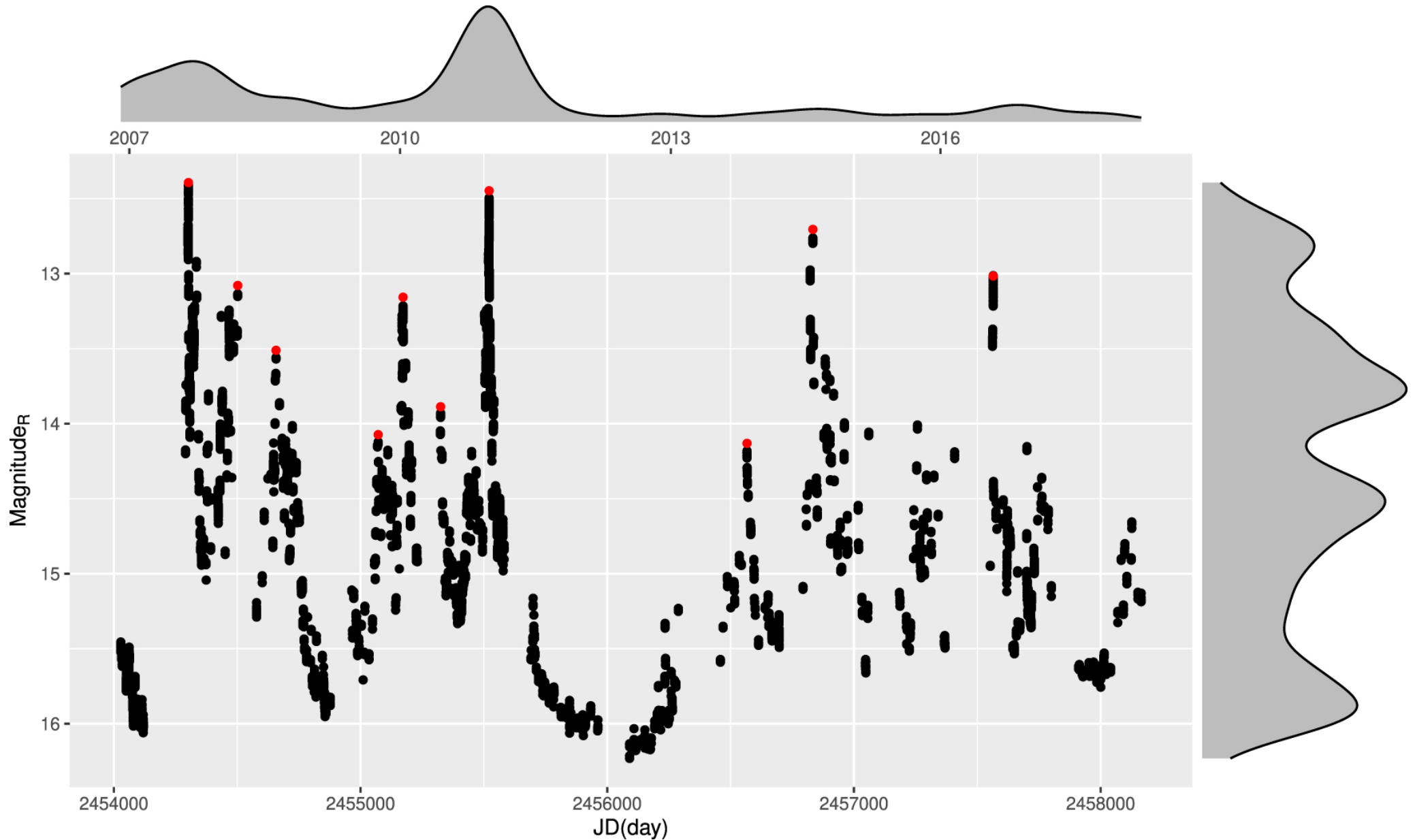
Figure 1. from Optical Photometry of the Quasar 3C 454.3 during the Period 2006–2018 and the Long-term Periodicity Analysis null 2021 APJS 253 10 doi:10.3847/1538-4365/abd32d https://dx.doi.org/10.3847/1538-4365/abd32d © 2021. The American Astronomical Society. All rights reserved.
