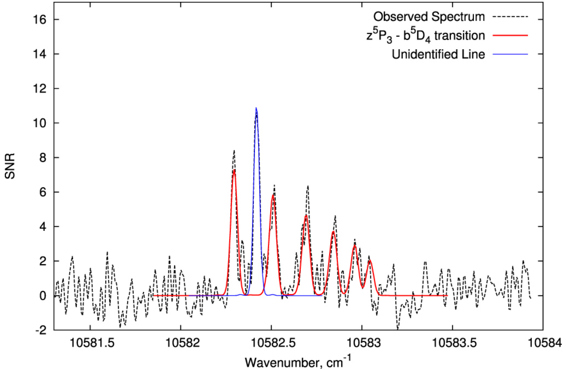
Figure 1. from The Spectrum and Term Analysis of Singly Ionized Manganese null 2021 APJS 252 10 doi:10.3847/1538-4365/abc75f http://dx.doi.org/10.3847/1538-4365/abc75f © 2021. The American Astronomical Society. All rights reserved.
