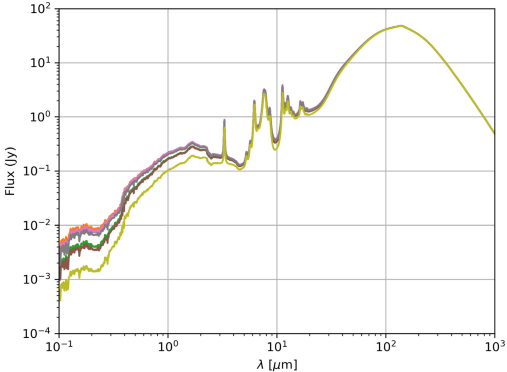
Figure 8. from POWDERDAY: Dust Radiative Transfer for Galaxy Simulations null 2021 APJS 252 12 doi:10.3847/1538-4365/abc487 http://dx.doi.org/10.3847/1538-4365/abc487 © 2021. The American Astronomical Society. All rights reserved.
