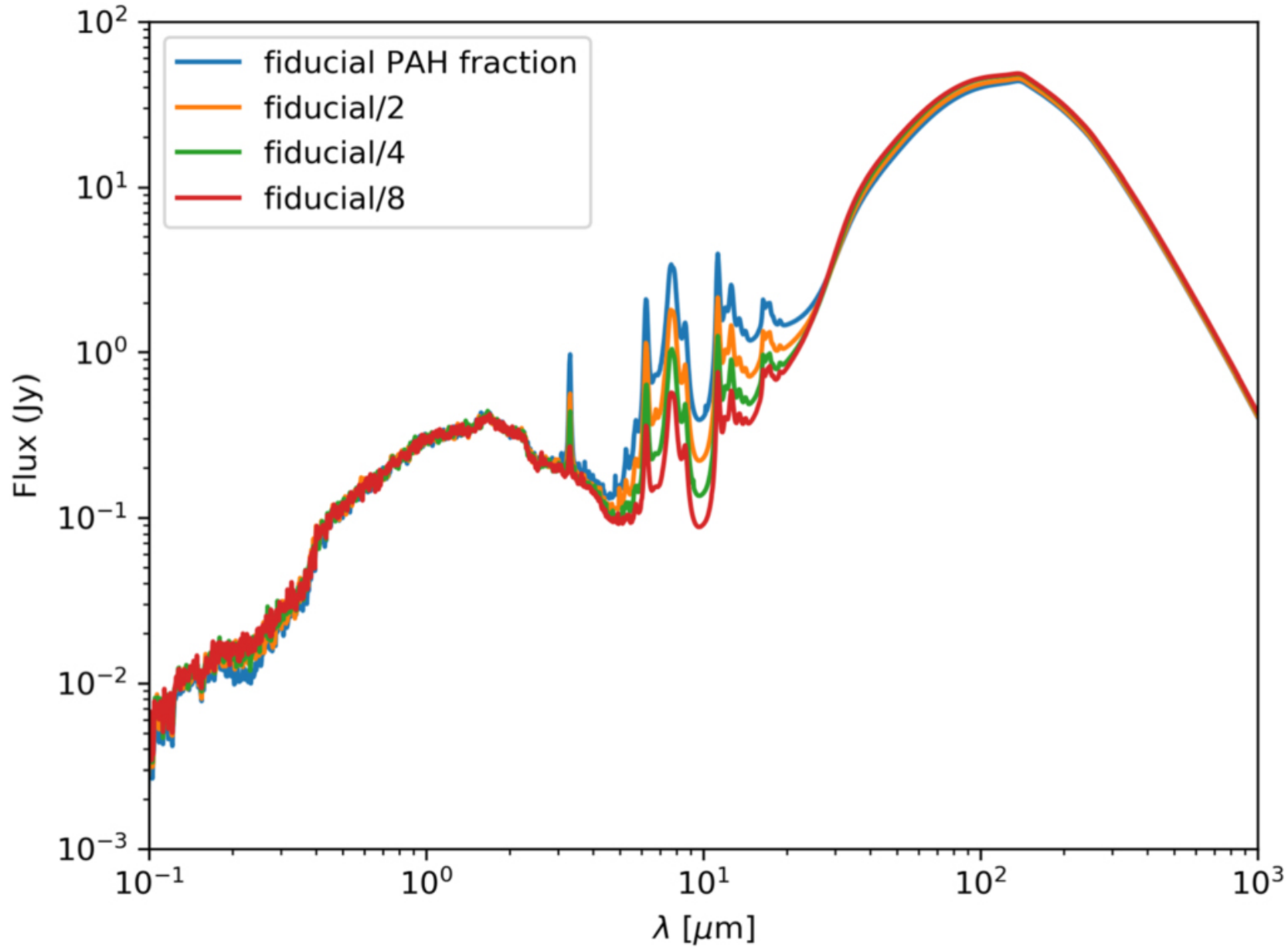
Figure 5. from POWDERDAY: Dust Radiative Transfer for Galaxy Simulations null 2021 APJS 252 12 doi:10.3847/1538-4365/abc487 http://dx.doi.org/10.3847/1538-4365/abc487 © 2021. The American Astronomical Society. All rights reserved.
