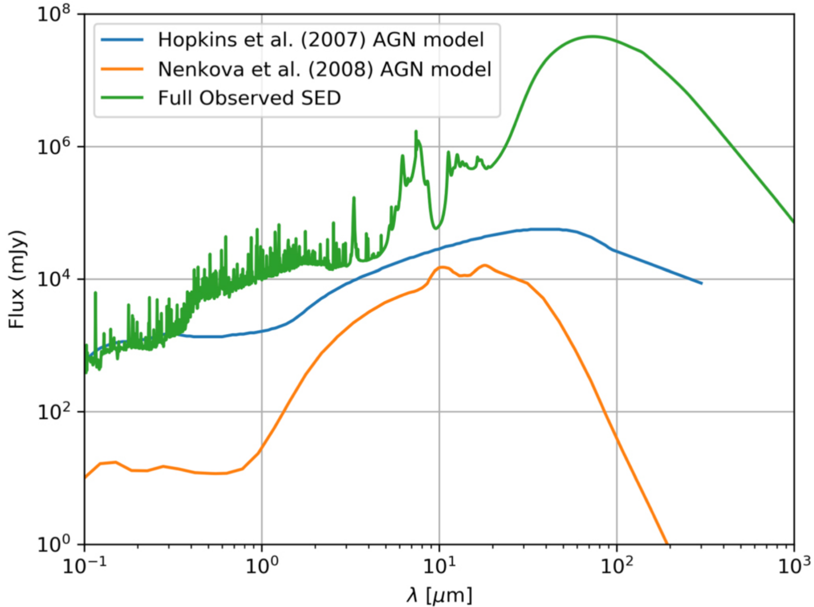
Figure 3. from POWDERDAY: Dust Radiative Transfer for Galaxy Simulations null 2021 APJS 252 12 doi:10.3847/1538-4365/abc487 http://dx.doi.org/10.3847/1538-4365/abc487 © 2021. The American Astronomical Society. All rights reserved.
