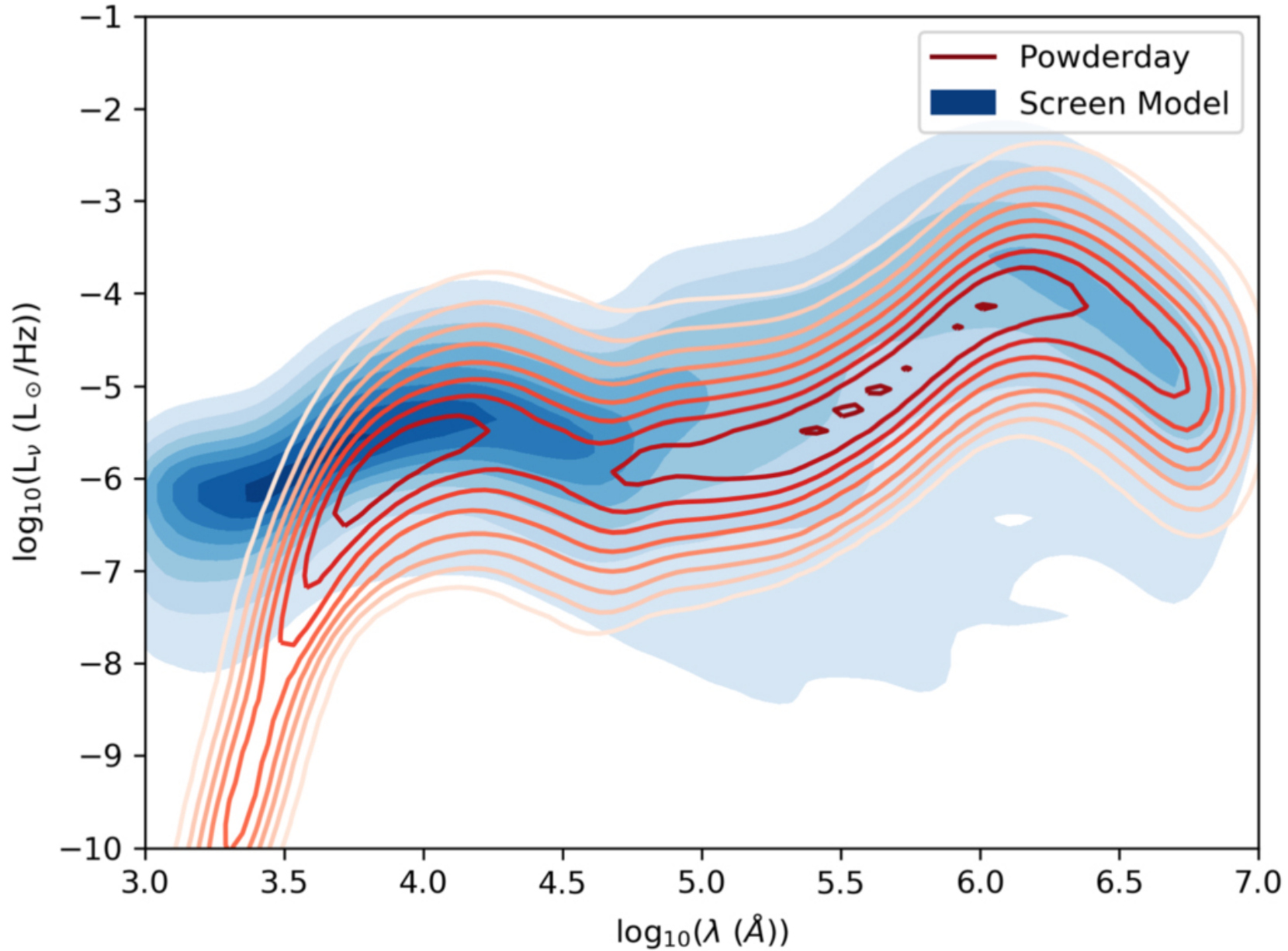
Figure 15. from POWDERDAY: Dust Radiative Transfer for Galaxy Simulations null 2021 APJS 252 12 doi:10.3847/1538-4365/abc487 http://dx.doi.org/10.3847/1538-4365/abc487 © 2021. The American Astronomical Society. All rights reserved.
