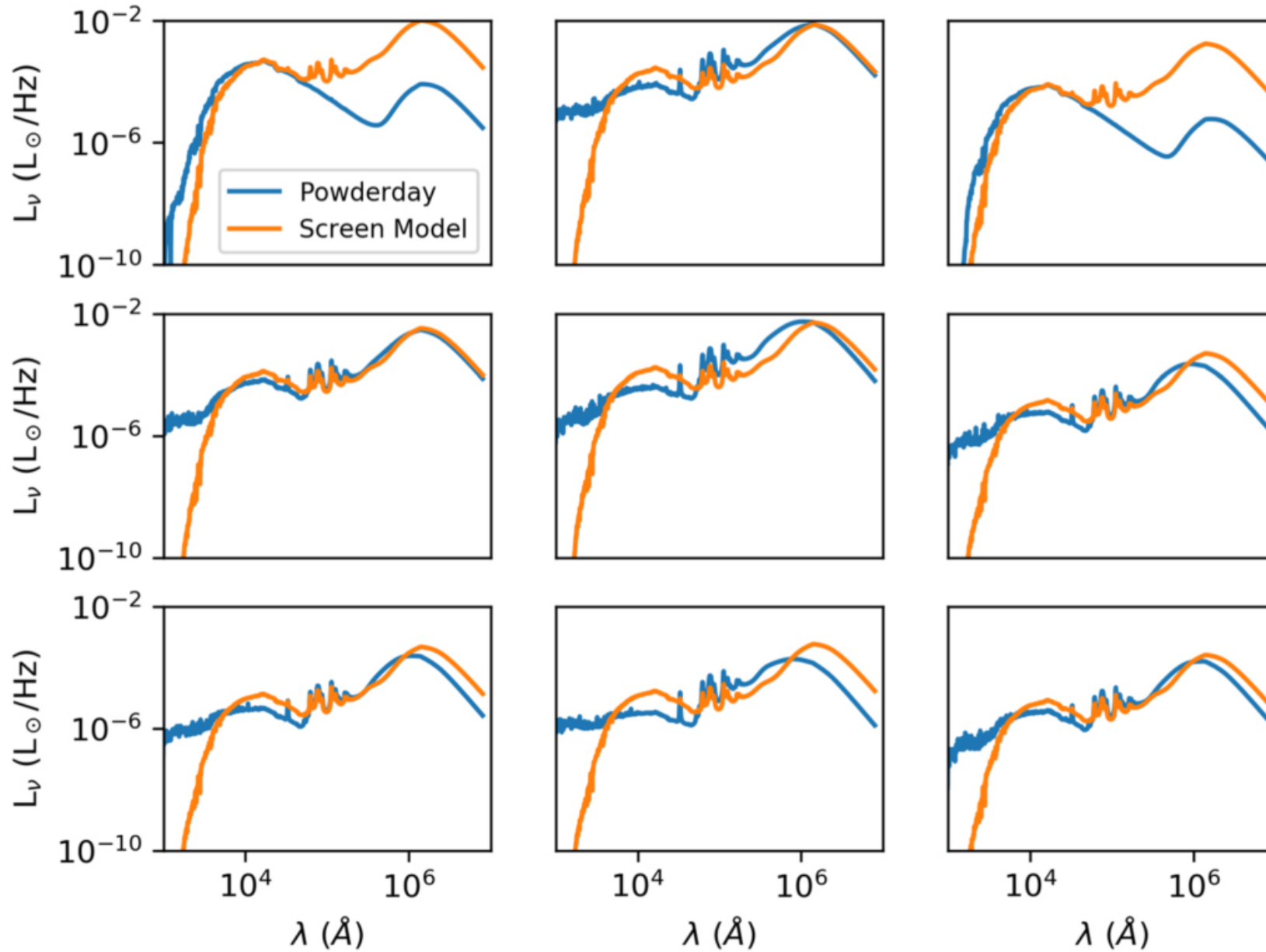
Figure 14. from POWDERDAY: Dust Radiative Transfer for Galaxy Simulations null 2021 APJS 252 12 doi:10.3847/1538-4365/abc487 http://dx.doi.org/10.3847/1538-4365/abc487 © 2021. The American Astronomical Society. All rights reserved.
