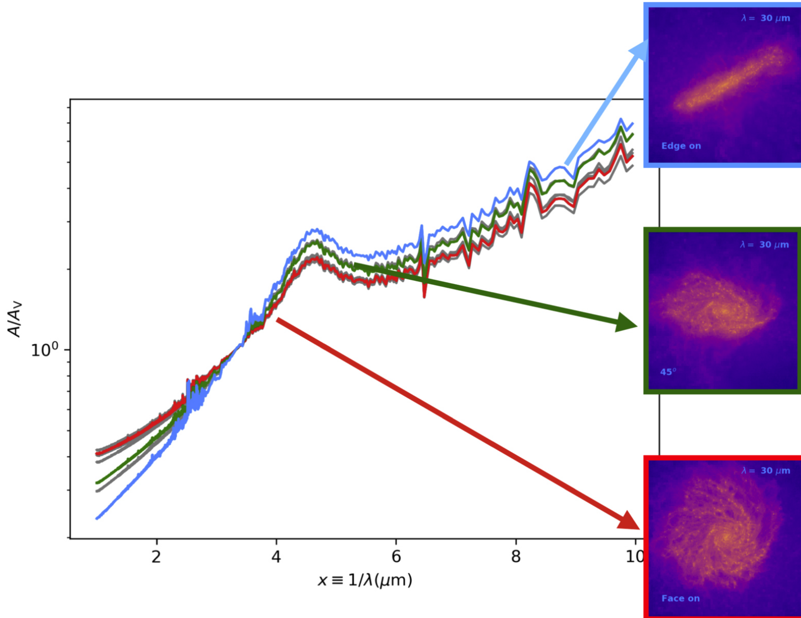
Figure 13. from POWDERDAY: Dust Radiative Transfer for Galaxy Simulations null 2021 APJS 252 12 doi:10.3847/1538-4365/abc487 http://dx.doi.org/10.3847/1538-4365/abc487 © 2021. The American Astronomical Society. All rights reserved.
