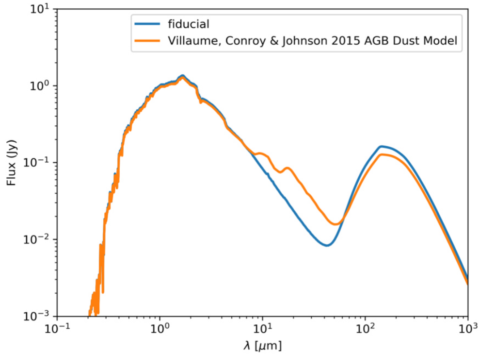
Figure 12. from POWDERDAY: Dust Radiative Transfer for Galaxy Simulations null 2021 APJS 252 12 doi:10.3847/1538-4365/abc487 http://dx.doi.org/10.3847/1538-4365/abc487 © 2021. The American Astronomical Society. All rights reserved.
