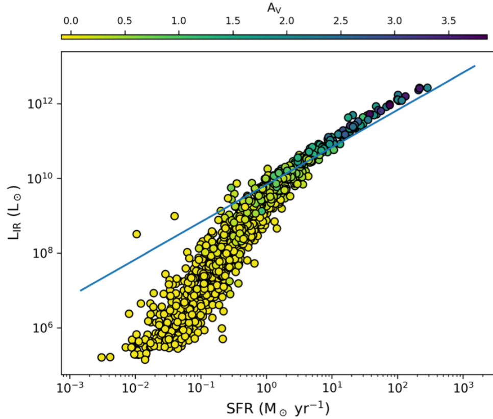
Figure 11. from POWDERDAY: Dust Radiative Transfer for Galaxy Simulations null 2021 APJS 252 12 doi:10.3847/1538-4365/abc487 http://dx.doi.org/10.3847/1538-4365/abc487 © 2021. The American Astronomical Society. All rights reserved.
