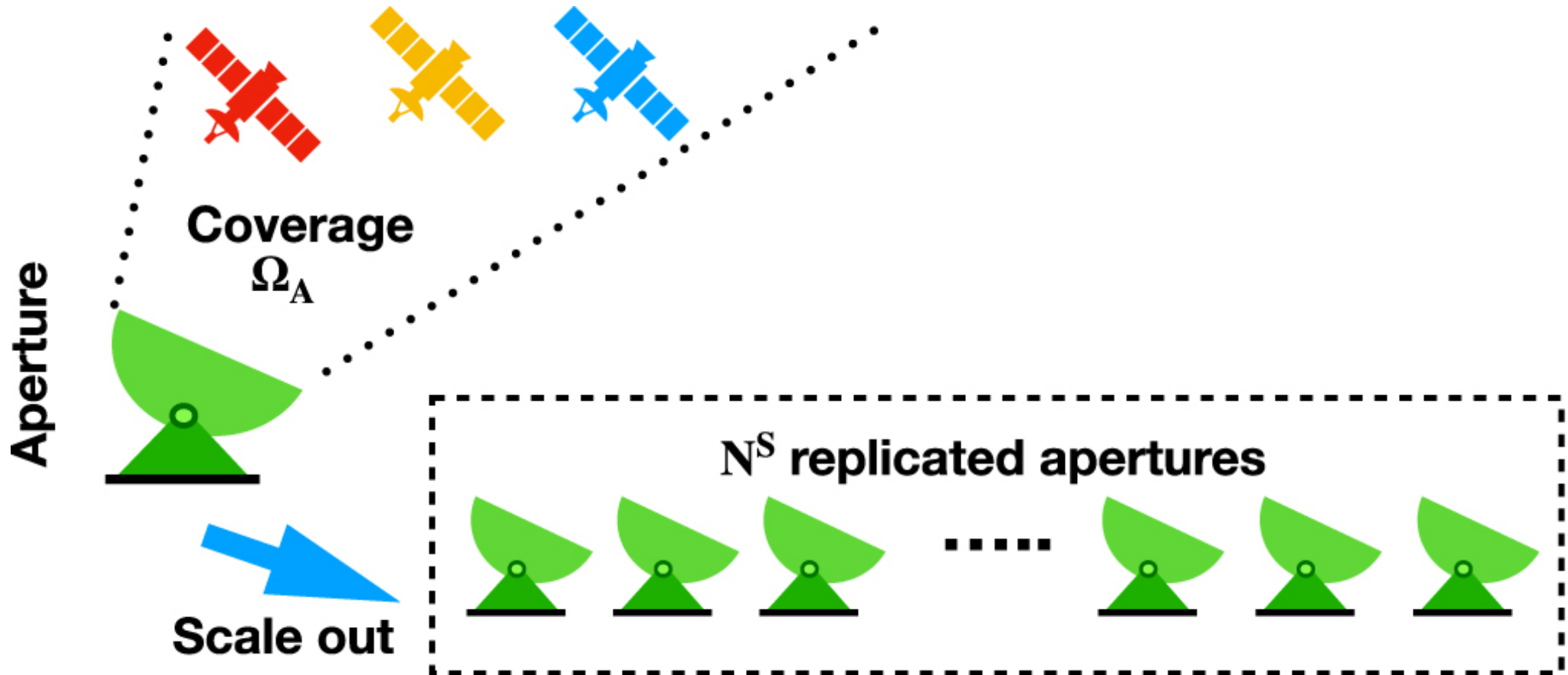
Figure 2. from Challenges in Scientific Data Communication from Low-mass Interstellar Probes null 2020 APJS 249 36 doi:10.3847/1538-4365/aba126 https://dx.doi.org/10.3847/1538-4365/aba126 © 2020. The American Astronomical Society. All rights reserved.
