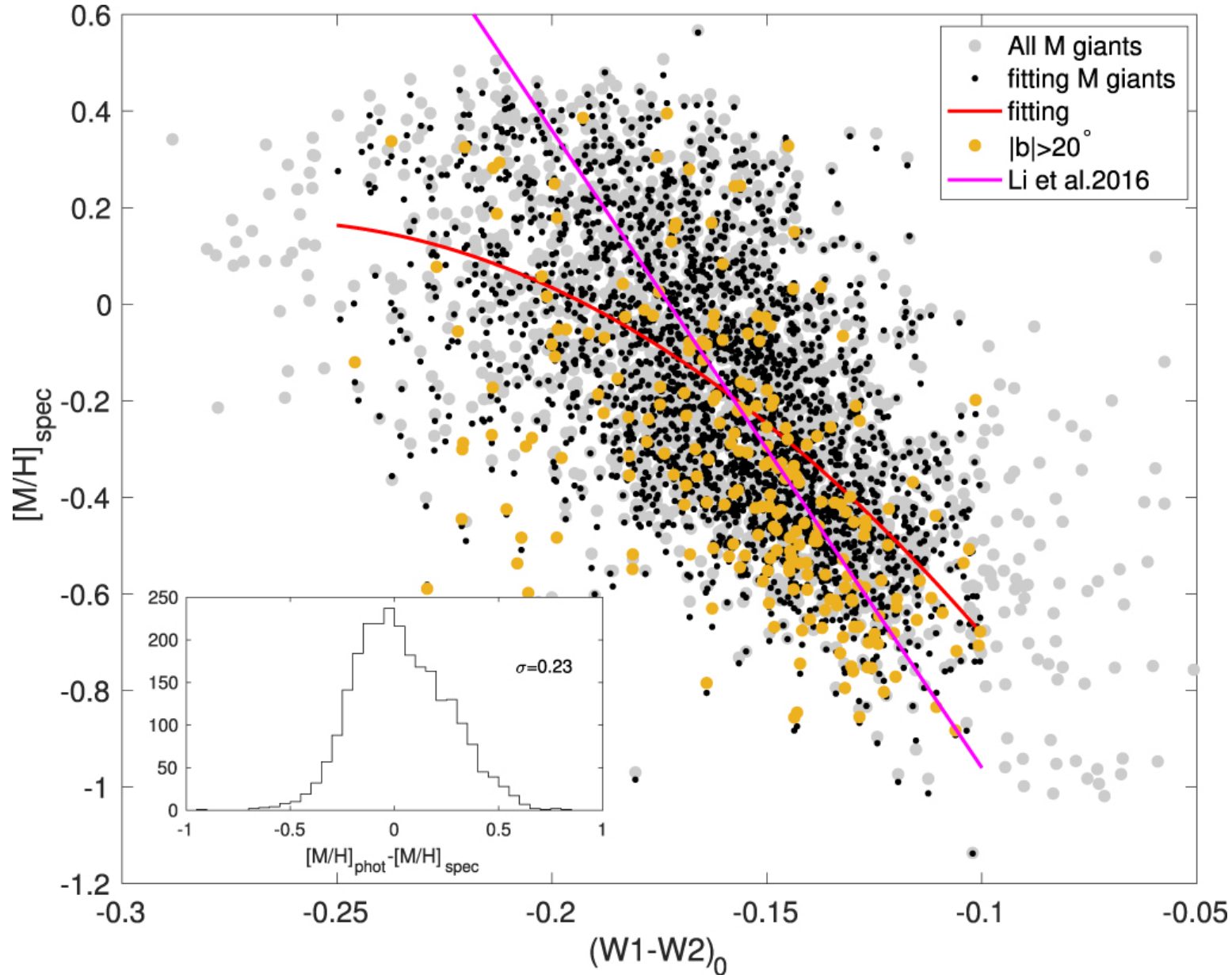
Figure 7. from Value-added Catalogs of M-type Stars in LAMOST DR5 null 2019 APJS 244 8 doi:10.3847/1538-4365/ab3859 http://dx.doi.org/10.3847/1538-4365/ab3859 © 2019. The American Astronomical Society. All rights reserved.
