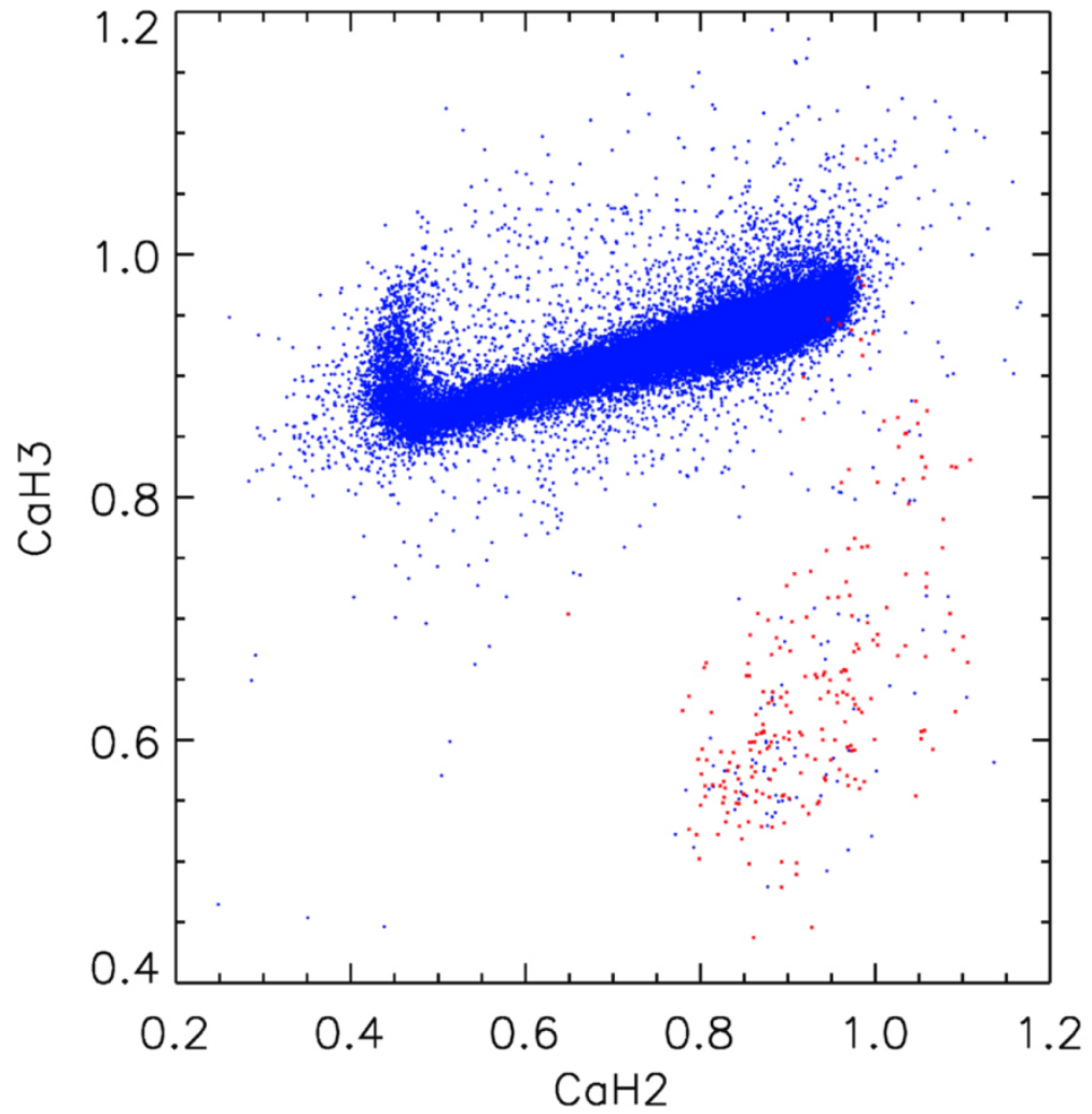
Figure 5. from Value-added Catalogs of M-type Stars in LAMOST DR5 null 2019 APJS 244 8 doi:10.3847/1538-4365/ab3859 http://dx.doi.org/10.3847/1538-4365/ab3859 © 2019. The American Astronomical Society. All rights reserved.
