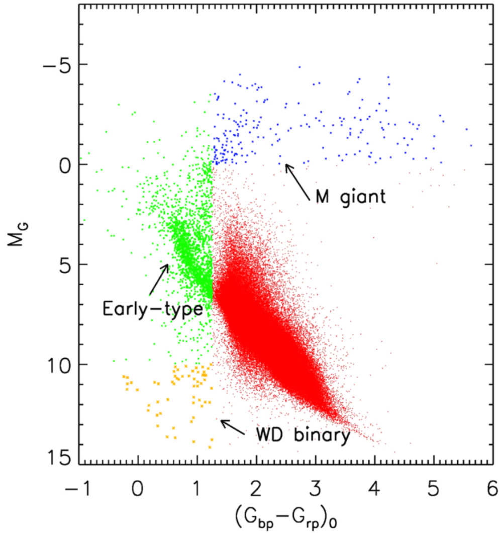
Figure 4. from Value-added Catalogs of M-type Stars in LAMOST DR5 null 2019 APJS 244 8 doi:10.3847/1538-4365/ab3859 http://dx.doi.org/10.3847/1538-4365/ab3859 © 2019. The American Astronomical Society. All rights reserved.
