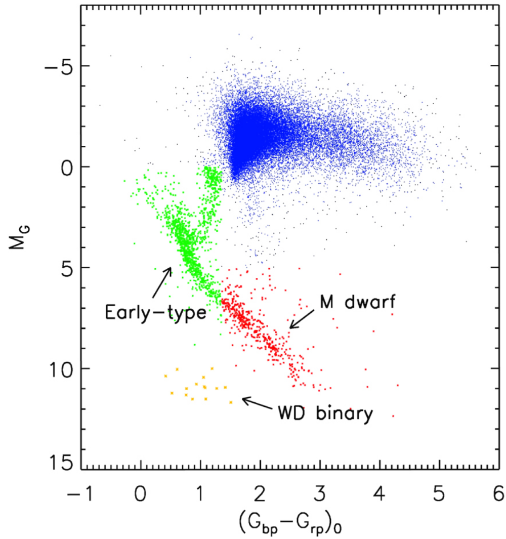
Figure 2. from Value-added Catalogs of M-type Stars in LAMOST DR5 null 2019 APJS 244 8 doi:10.3847/1538-4365/ab3859 http://dx.doi.org/10.3847/1538-4365/ab3859 © 2019. The American Astronomical Society. All rights reserved.
