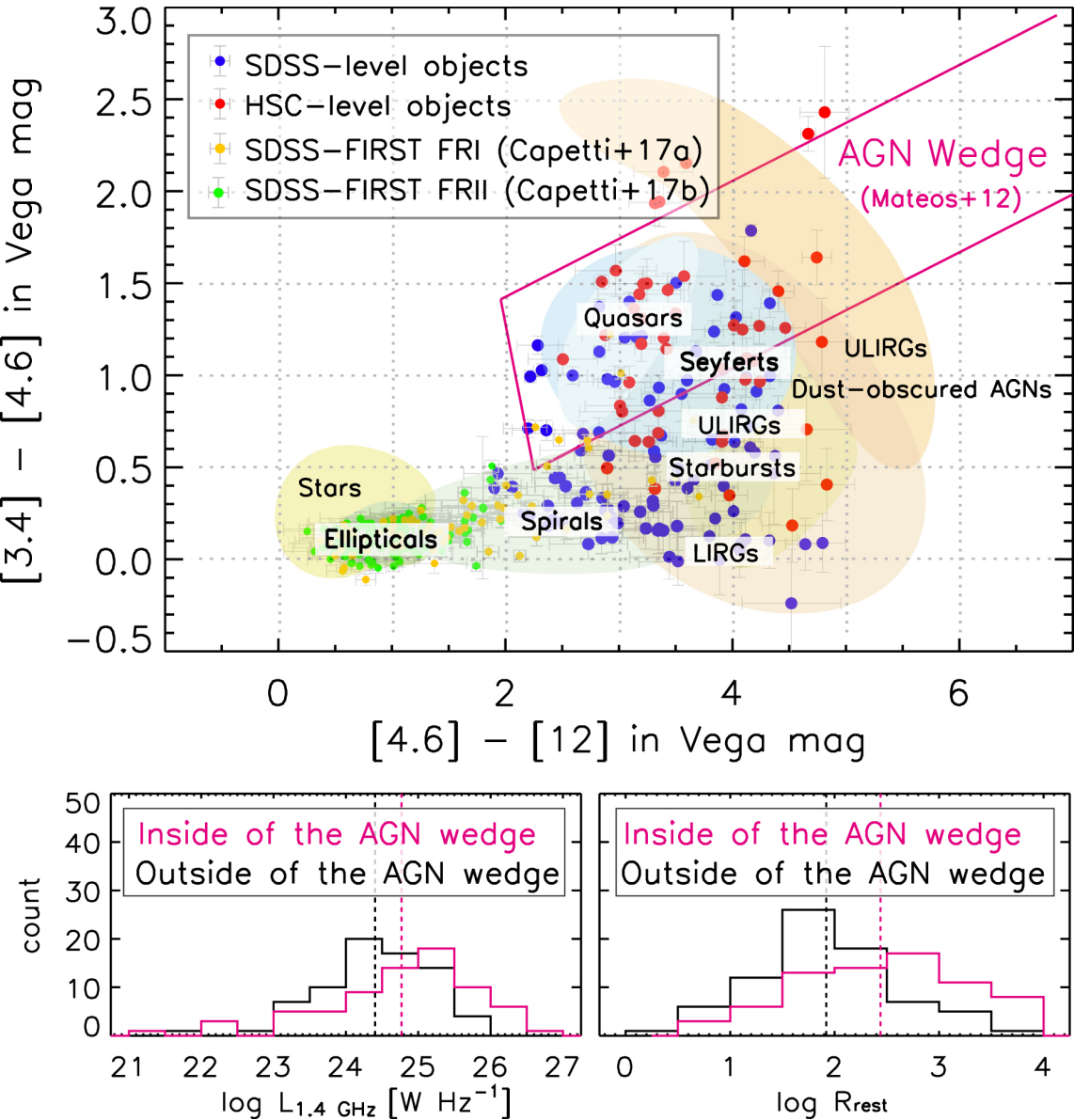
Figure 7. from A Wide and Deep Exploration of Radio Galaxies with Subaru HSC (WERGS). II. Physical Properties Derived from the SED Fitting with Optical, Infrared, and Radio Data null 2019 APJS 243 15 doi:10.3847/1538-4365/ab238d https://dx.doi.org/10.3847/1538-4365/ab238d © 2019. The American Astronomical Society. All rights reserved.
